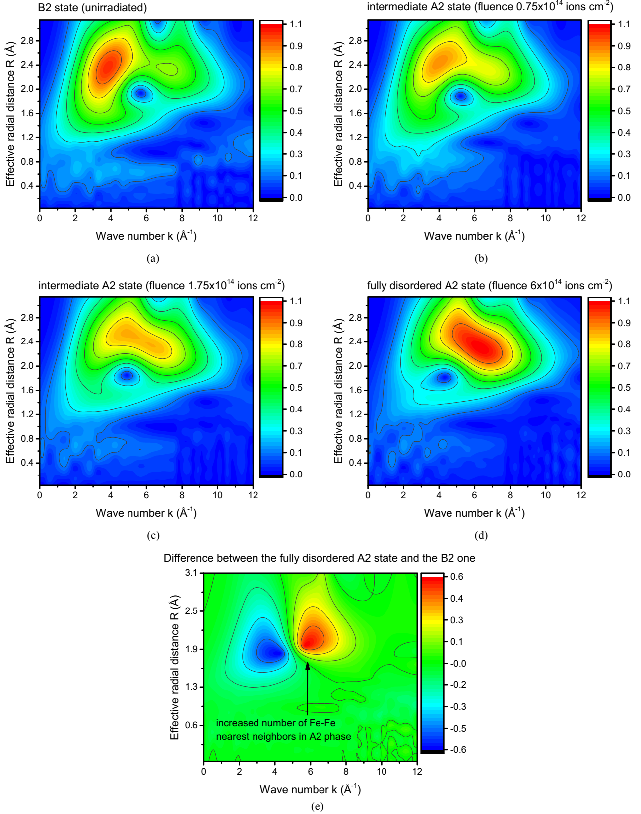
FIG. 3. Normalized wavelet transforms WT(R, k) of k\chi(k) of the annealed (unirradiated) sample (a), the “disorder-gradient” sample irradiated with fluences of 0.75 \times 10^{14} \text{ ions cm}^{-2} (b) and 1.75 \times 10^{14} \text{ ions cm}^{-2} (c), and the sample uniformly irradiated with the highest fluence of 6 \times 10^{14} \text{ ions cm}^{-2} (d). The radial distance axis ( R ) represents only an effective distance since the wavelet transform function WT(R, k) is not phase corrected; a relocation of WT(R, k) maxima along the B2 \rightarrow A2 transition is clearly visible. The difference of the WT presented in panels (d) and (a) is shown in panel (e).
