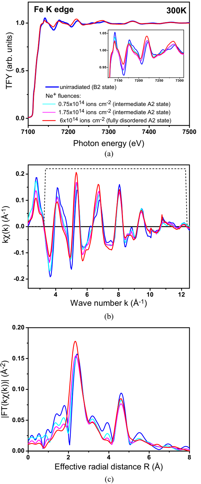
FIG. 2. (a) Experimental EXAFS spectra of the studied samples recorded at the Fe K edge and room temperature, (b) extracted EXAFS oscillations \chi(k) weighted with k , and (c) their Fourier transforms |\text{FT}(k\chi(k))(R)| . The degree of the chemical disorder increases from blue to red; with an increasing of the chemical disorder the minimum of |\text{FT}(k\chi(k))(R)| at R = 2 \text{ \AA} vanishes.
