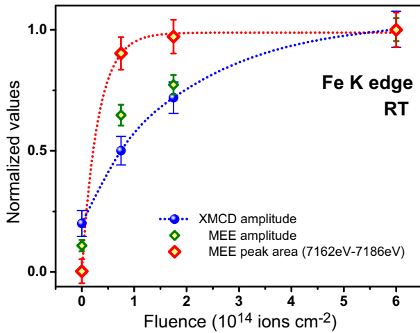
FIG. 9. Fluence dependence of the XMCD and MEE peak amplitude and the integrated MEE signal (7162–7186 eV) for the ordered (B2) and the disordered (A2) states of \text{Fe}_{60}\text{Al}_{40} recorded at the Fe K edge at RT. Dotted lines are guides for the eyes.
