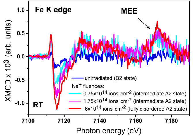
FIG. 8. XMCD spectra for the ordered ( B2 ) and the disordered ( A2 ) states of \text{Fe}_{60}\text{Al}_{40} recorded at the Fe K edge at RT; the magnetic MEE peaks are clearly visible only for the A2 states.
