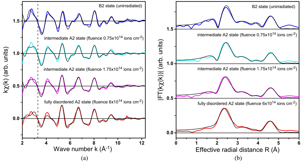
FIG. 4. Experimental data (colored lines) together with fitting results (black lines) of EXAFS oscillations k\chi(k) (a) and related Fourier transforms |\text{FT}(k\chi(k))(R)| (not phase corrected) (b) for all studied samples. The curves for different samples are shifted vertically for convenience. The degree of the chemical disorder increases from the top to the bottom. The beginning of the window function used in the FT is showed by the vertical dashed line. The minimum of |\text{FT}(k\chi(k))(R)| at R = 2 \text{\AA} becomes less pronounced with increase of the chemical disorder and its magnitude is linked to the number of Al atoms in the first coordination shell of Fe absorber.
