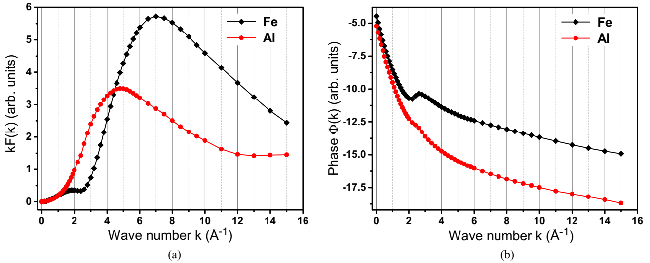
FIG. 1. (a) Calculated backscattering amplitudes F(k) weighted with k for Fe and Al atoms in \text{Fe}_{60}\text{Al}_{40} model structure using FEFF9. The peak positions are important for the interpretation of the further wavelet transforms \text{WT}(R, k) . (b) The calculated phase factors \Phi(k) of the backscattering Fe and Al atoms in the same model structure. The nonlinearity of \Phi(k) leads to the rotated maxima in the \text{WT}(R, k) plots.
