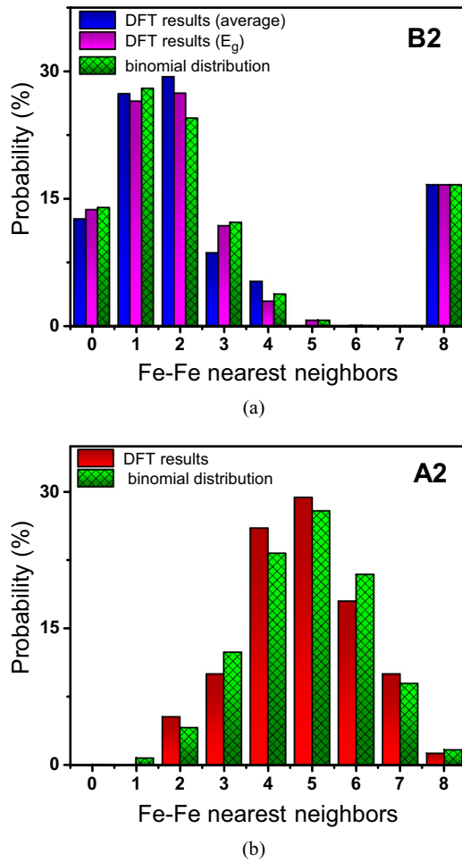
FIG. 6. The distributions of Fe-Fe nearest neighbors in the \text{Fe}_{60}\text{Al}_{40} model crystal for the chemically ordered B2 state in the local layer-wise configurations (averaged over all configurations and in the configuration with minimum ground-state energy E_g ) (a) and the chemically disordered A2 state (b) calculated by VASP. The ideal case of homogeneously distributed disorder is represented by binomial distribution.
