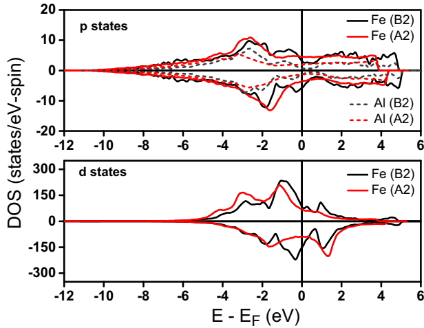
FIG. 7. Spin-resolved DOS for Fe and Al p states (top panel) and Fe d states (bottom panel) in B2 and A2 phases calculated by VASP.
