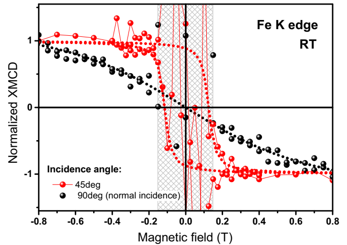
FIG. 10. Element-specific hysteresis loop measured by XMCD at the Fe K edge (7116 eV) for the sample irradiated with 1.75 \times 10^{14} ions \text{cm}^{-2} fluence at two different incident angles as indicated. Symbols represent the experimental data, and dotted lines are the corresponding fits by Langevin function used as guides for eyes. The patterned area relates to the signal instability region.
