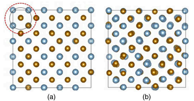
FIG. 5. Relaxed structures for the ordered B2 phase (a) and the fully disordered A2 phase (b) of an Fe-rich \text{Fe}_{60}\text{Al}_{40} model crystal (side view). The first and the second coordination shells of Fe atoms are schematically represented by dotted and dashed lines, respectively.
