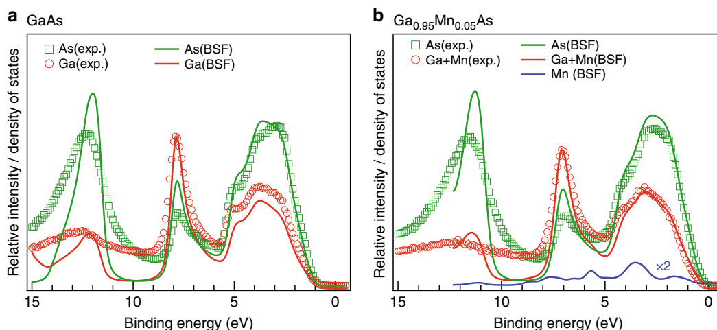
Fig. 5 Elemental projection of angle-integrated experimental data. Projections represent roughly the matrix-element weighted density-of-states of element-resolved components. Experimental data for a GaAs and b (Ga,Mn)As in a (-1-1-1) reflection geometry, with photon energy of \sim 2.7 keV and integrated over the whole-acceptance angle of analyzer are shown as empty circles (red for Ga+Mn) and squares (green for As). The solid curves show element-projected calculated partial densities of states of Ga, As, or Ga+Mn, sites, including coherent potential approximation for the doped sample. The blue curve (whose intensity is multiplied by 2) shows the theoretical projection onto Mn only
