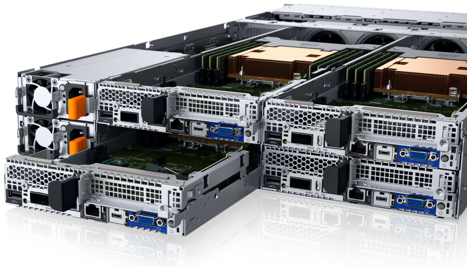
Figure 3: Example of a Dell C6320P server system. The model used in the JURECA Booster slightly deviates from the shown version due to the utilized processor type. Copyright: Dell Technologies.
