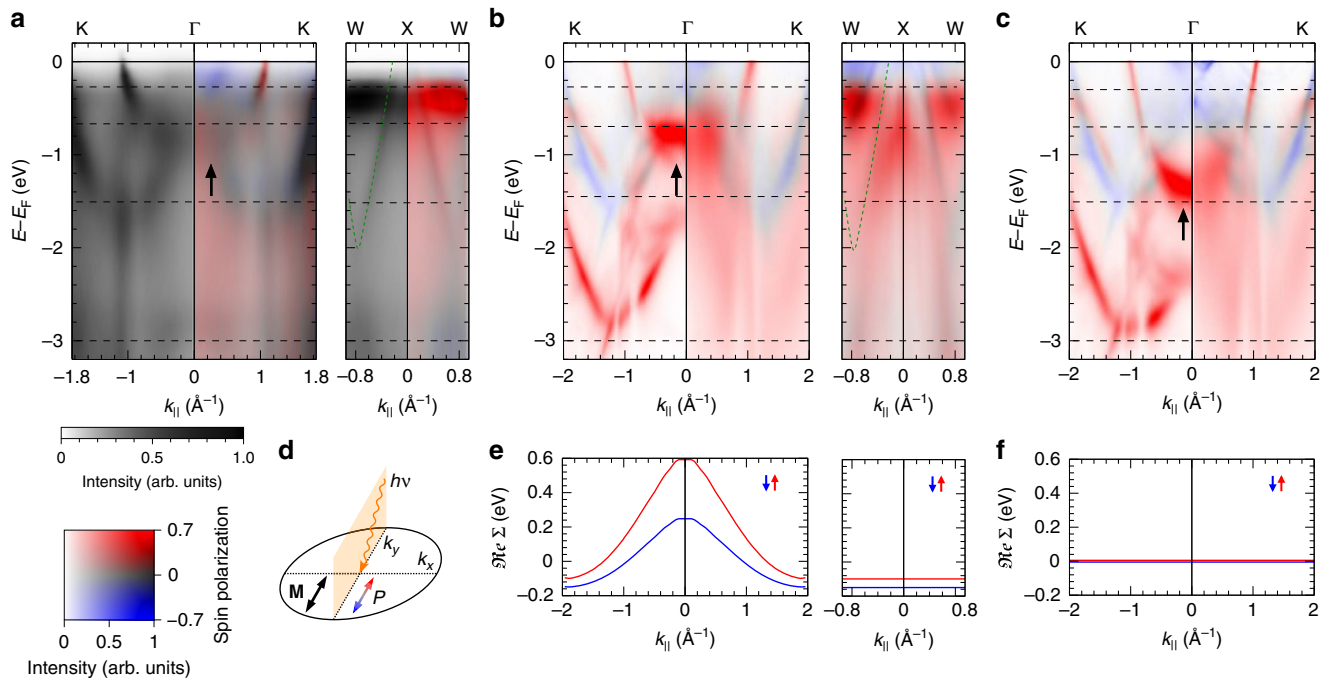
Fig. 2 Spin-resolved band dispersion maps. a Dispersion of cobalt bands along the K- \Gamma -K and W-X-W directions as function of binding energy ( E - E_F ), measured at h\nu = 50 eV. The left half in a shows the spin-averaging experiment on a grey intensity scale, and the right half the spin-resolved experiment in the same 2D colour code as in Fig. 1. Dashed horizontal lines indicate energies of 2D momentum maps in Fig. 4. b Calculated spin-resolved photoemission intensities corresponding to a using momentum-dependent corrections for the band renormalization \Re\Sigma_\sigma(\mathbf{k}) as in e , and constant (left half) or E -dependent broadening \Im\Sigma_\sigma(E) (right half). Dashed curves indicate faint band positions as guide to the eye. c Calculation using a constant \Re\Sigma as for in f . The bottom of the majority electron parabola (see solid arrows) lies too deep, compared with the experiment in a and calculation in b . The right half of panel c uses an energy dependent \Im\Sigma_\sigma(E) following DMFT calculations from Ref. 11 , which underestimates broadening close to E_F . d Photoemission geometry used both, in experiment and theory: The photon beam is incident along the positive k_y direction with 25° towards the surface, magnetization \mathbf{M} and polarization \mathbf{P} are in-plane along k_y .
