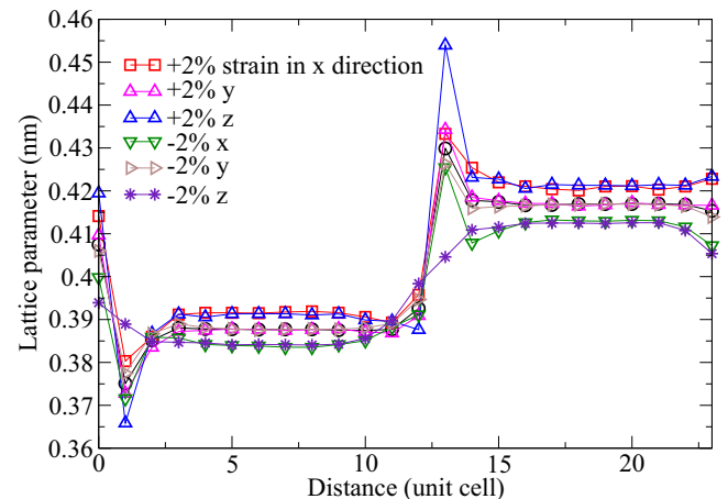
FIG. 4. Variation of lattice parameter across the domain wall with 2% lattice strains in different directions. The domain structure is especially sensitive to strains in the z direction.
