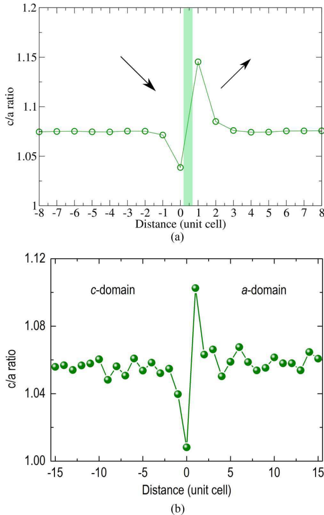
FIG. 3. Variation of the c/a ratio across the domain wall as found in (a) first-principles calculation on \text{PbTiO}_3 and (b) experimental measurements on PZT 10/90 thin film.
