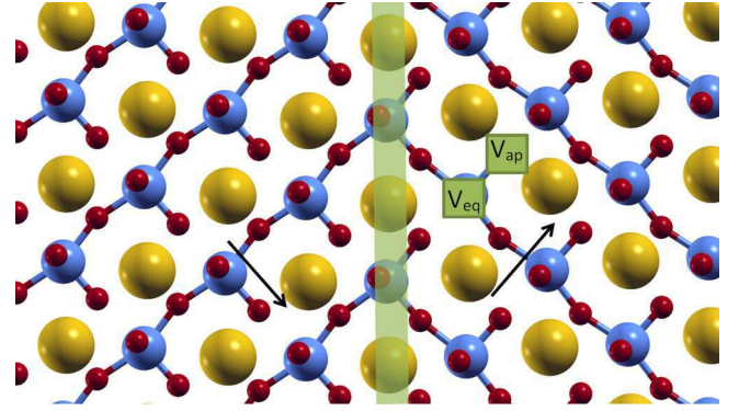
FIG. 6. Schematic showing the ground-state positions of the apical oxygen vacancy ( V_{ap} ) and equatorial oxygen vacancy ( V_{eq} ). The large yellow spheres are lead atoms, blue sphere are titanium, small red spheres are oxygen. The domain wall plane is represented by the vertical green region across the middle of the figure. Black arrows in the figure show the direction of polarization in each domain.
