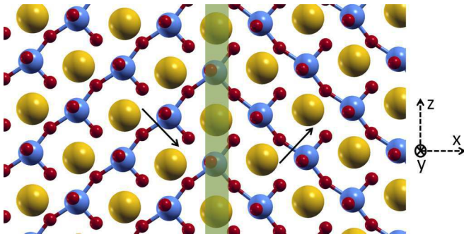
FIG. 1. Schematic showing the relaxed supercell of the 90^\circ domain wall. The large yellow spheres are lead atoms, blue sphere are titanium, and small red spheres are oxygen. The domain wall plane is represented by the vertical green region across the middle of the figure. Black arrows in the figure show the direction of polarization in each domain. The x , y , and z directions are represented by the dashed lines on the right.
