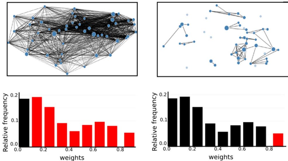
FIGURE 13 | High thresholds on graph edges cause the graphs to dissociate. (Upper Panel) , Illustration of graph with edge weights larger then 0.1 ( w_{\min} > 0.1 , Left ) and larger then 0.9 ( w_{\min} > 0.9 , Right ). In the according weight histograms (Lower Panel) the red bars correspond to the edges drawn in the upper graph. Edges corresponding to the black bars are not shown.
