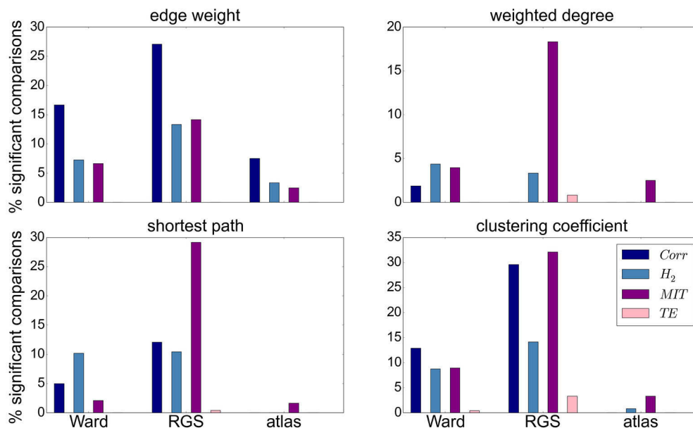
FIGURE 6 | Significant relationships in graph metrics between health conditions dependent on edge definition methods. Percentage of significant differences for each clustering technique [Ward (left), RGS (middle), atlas (right)] for each class of edge definition method clustering method [Corr (dark blue), H2 (light blue), MIT (purple), TE (pink)] for averaged graph properties: edge weight ( Upper Left ), weighted degree ( Upper Right ), shortest path ( Lower Left ) and clustering coefficient ( Lower Right ). Fraction of significant differences are calculated for each health condition over all graphs constructed with the corresponding clustering and edge techniques including all variants in parameters, thresholds and rich-club sub-graphs. Significance is calculated as in the lower panel of Figure 4 .
