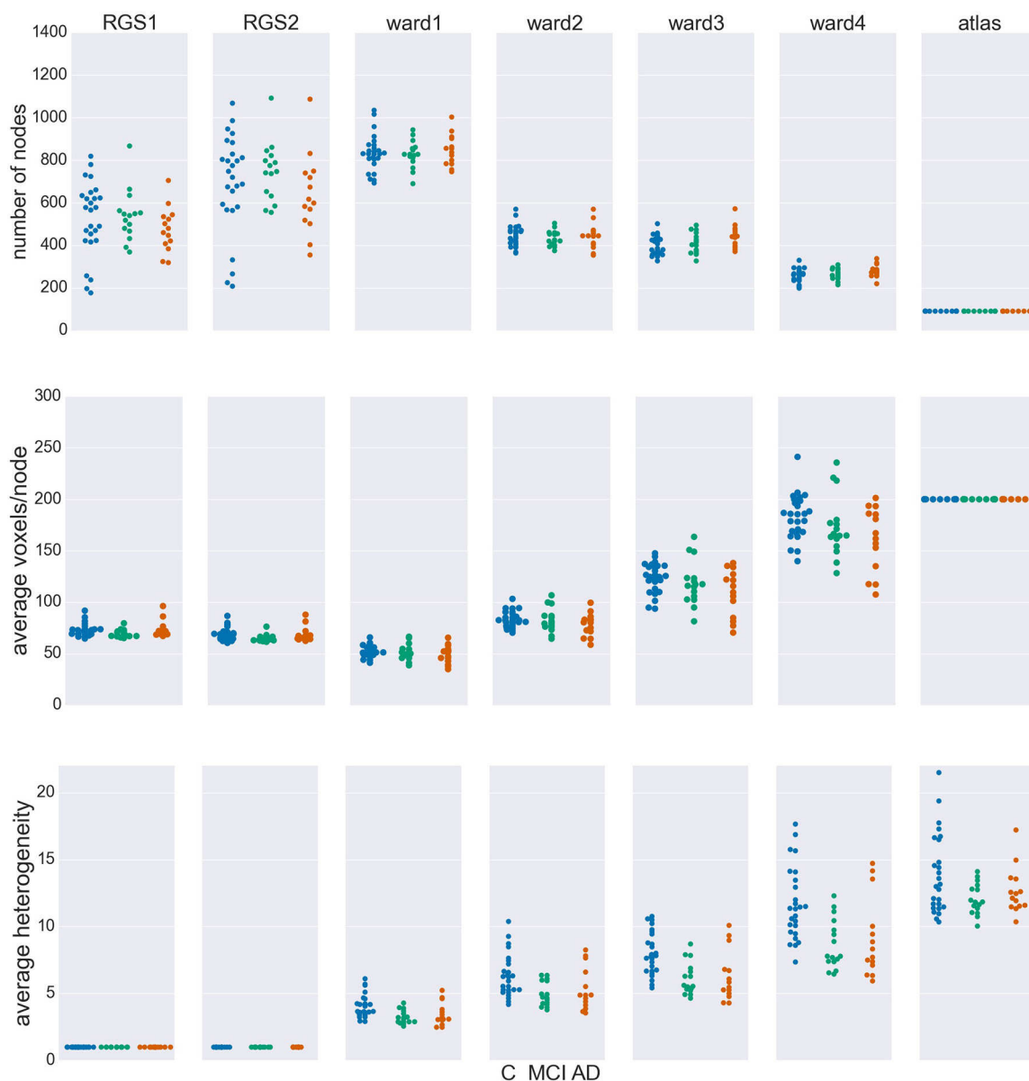
FIGURE 2 | Node properties across different clustering algorithms. For each of the seven clustering methods detailed in section 5.3 and Table 3 , and each subject categorized in the health conditions: control (C, blue dots), mild cognitive impairment (MCI, green dots), and Alzheimer's disease (AD, orange dots) we calculate the total number of nodes/clusters generated ( Upper Panel ), the average number of voxels per node ( Middle Panel ), and the average cluster heterogeneity ( Lower Panel ).
