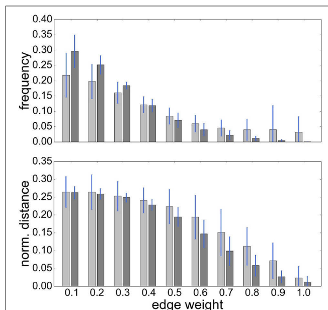
FIGURE 3 | RGS clustering yields stronger long-range connections than Ward clustering. Frequency ( Upper Panel ) and connection distance normalized to maximum graph distance ( Lower Panel ) across a range of graph edge weights calculated based on BcorU1 for RGS1 (light gray bars) and ward2 (dark gray) clustering. Mean values and standard deviation (blue vertical lines) are calculated across single histogram values of all subjects independent of health condition.
