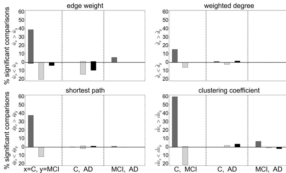
FIGURE 5 | Significant relationships in graph metrics between health conditions dependent on clustering methods. Percentage of significant differences for each clustering method RGS (dark gray), Ward (light gray), and atlas (black) for different averaged graph properties: edge weight ( Upper Left ), weighted degree ( Upper Right ), shortest path ( Lower Left ) and clustering coefficient ( Lower Right ). Fraction of significant differences are calculated for each health condition over all graphs constructed with the corresponding clustering including all variants in parameters, edge definition techniques, thresholds and rich club sub-graphs. The abscissa labels show which pairs of health conditions are compared (C-MCI, C-AD, MCI-AD) and the ordinate labels the direction of the significant differences (“<,” “>”). Significance is calculated as in the lower panel of Figure 4 .
