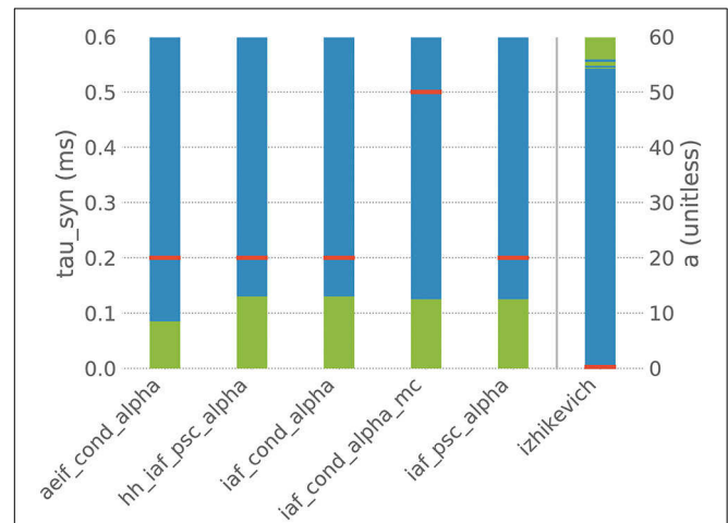
FIGURE 4 | Results of the stiffness test for six neuron models from NEST. Red bars indicate the default value of the selected parameter in NEST, blue indicates the value range in which the system of ODEs evaluates as non-stiff, green indicates the range in which it evaluates as stiff. aeif_cond_alpha is a conductance-based adaptive exponential integrate-and-fire model with alpha-shaped postsynaptic conductances, hh_psc_alpha a Hodgkin-Huxley type model with alpha-shaped postsynaptic currents, iaif_cond_alpha a conductance-based integrate-and-fire neuron with alpha-shaped postsynaptic conductances, iaif_cond_alpha_mc a conductance-based integrate-and-fire neuron with alpha-shaped postsynaptic conductances and multiple compartments, iaif_psc_alpha a current-based integrate-and-fire neuron with alpha-shaped postsynaptic currents and izhikevich the model dynamics proposed by Izhikevich (2003). The test was applied to the ODE systems for varying values of the parameter \tau_{syn} of the first five models and for the parameter a of the last model.
