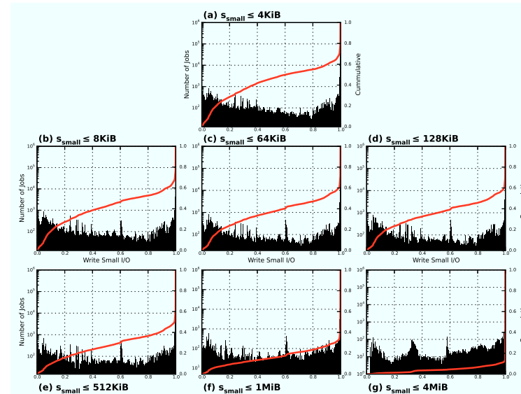
FIGURE 4.28: Percentage of small write I/O for analysed jobs computed using various s_{small} . (a) s_{small} < 4\text{KiB} , (b) s_{small} < 8\text{KiB} , (c) s_{small} < 64\text{KiB} , (d) s_{small} < 128\text{KiB} , (e) s_{small} < 512\text{KiB} , (f) s_{small} < 1\text{MiB} and (g) s_{small} < 4\text{MiB}
