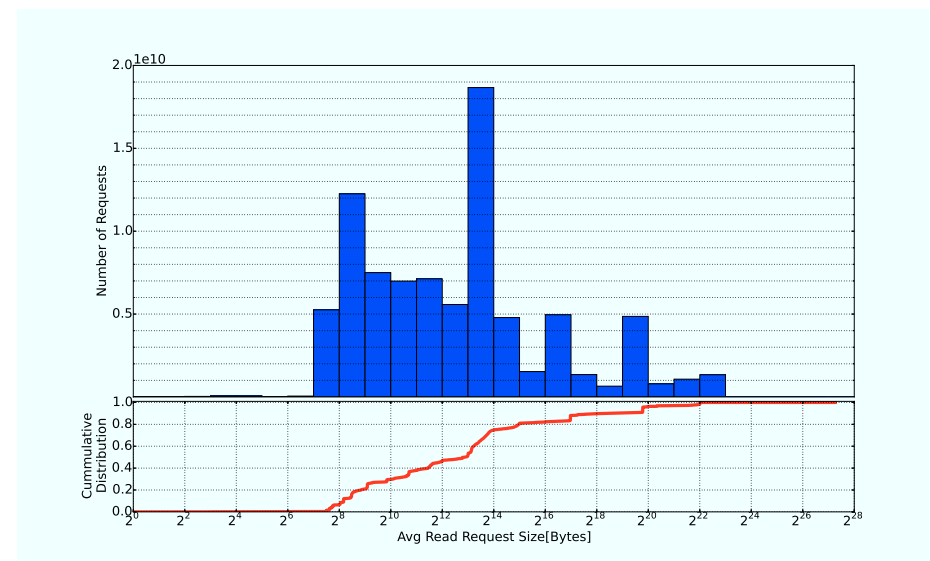
FIGURE 4.24: Distribution of read request sizes.
