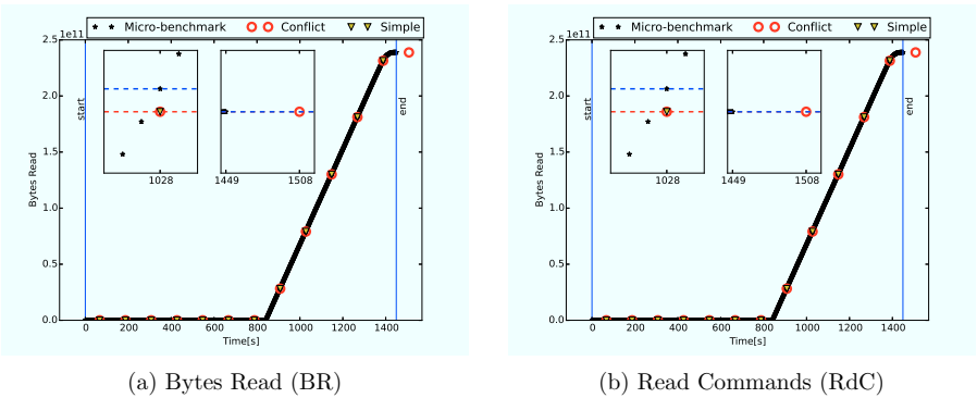
FIGURE 4.8: Bytes Read (BR) and Read Commands (RdC), for matching POSIX-I/O task-local files 1024KiB 32 node test to GPFS I/O logs.
