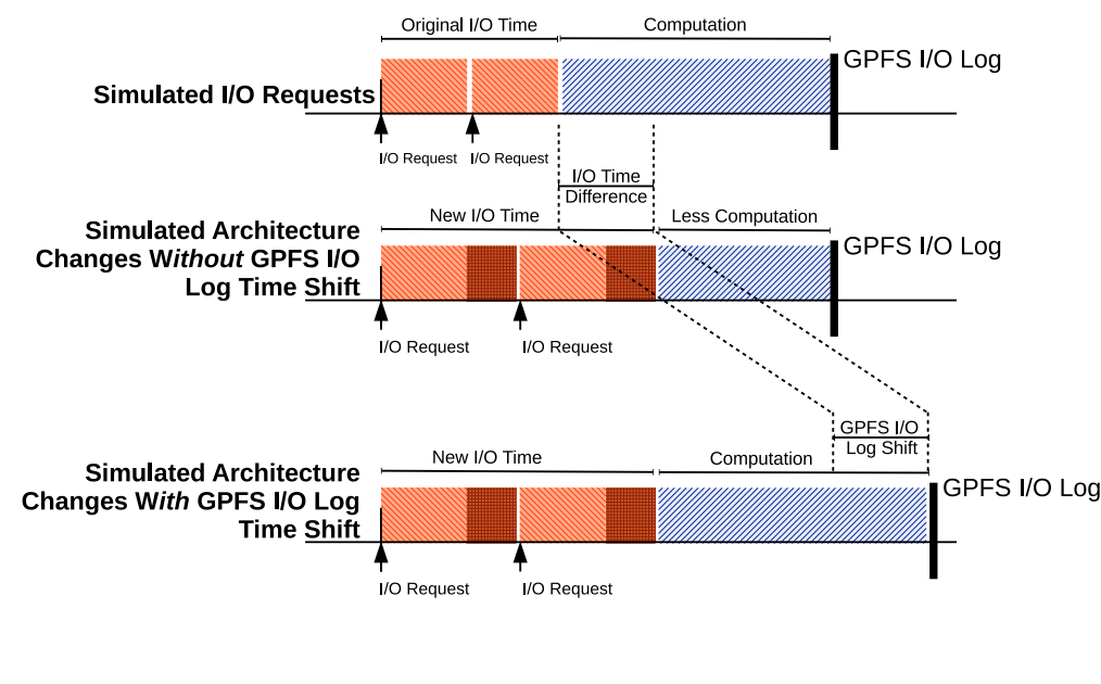
FIGURE 5.10: Time shifting GPFS I/O logs in the I/O model.
