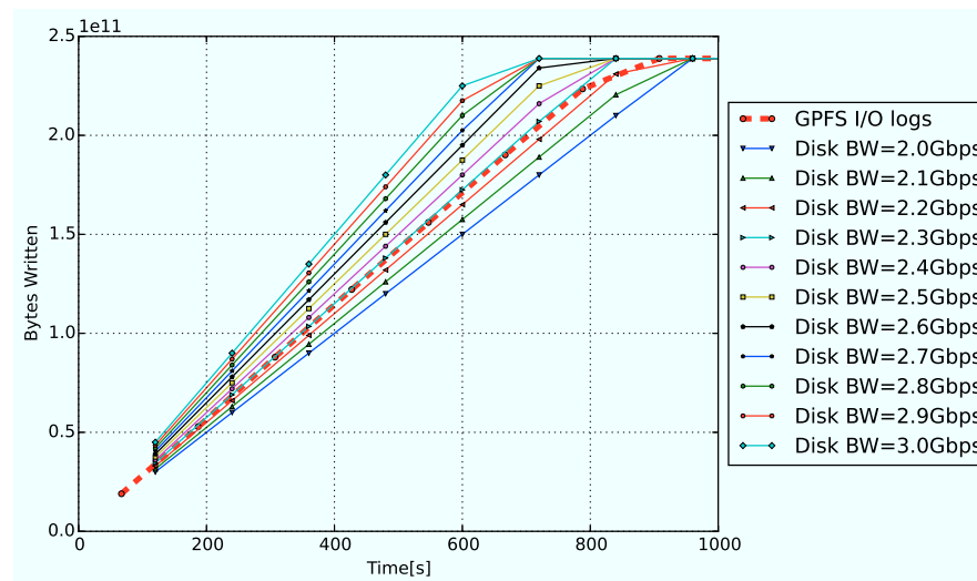
FIGURE B.2: Example of I/O model parameter fitting using I/O benchmark for write
