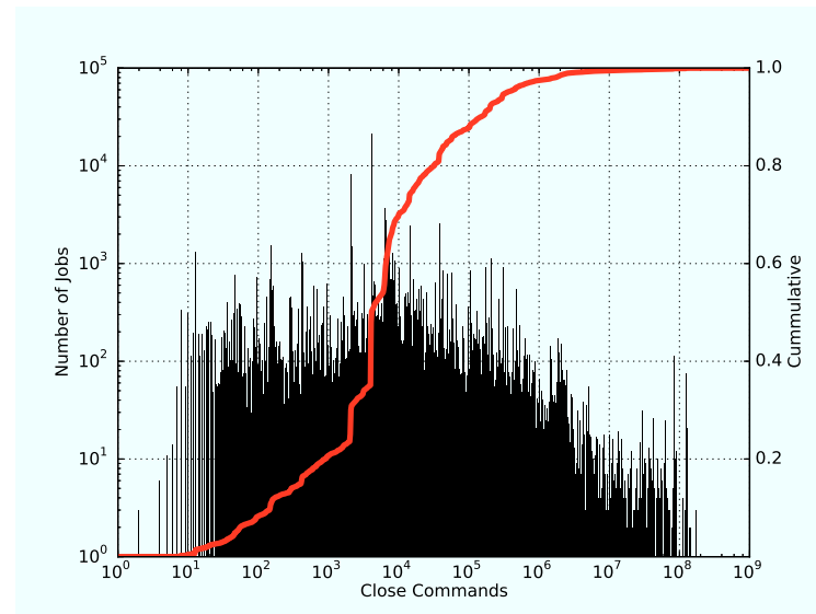
FIGURE 4.20: Close commands for analysed jobs.
