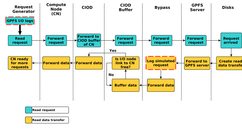
FIGURE 5.4: I/O model read flow graph.
