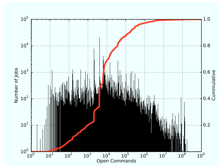
FIGURE 4.19: Open commands for analysed jobs.
