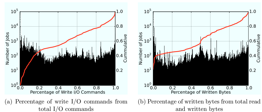
FIGURE 4.29: Percentage of write for analysed jobs
