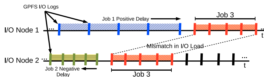
(b) Unsynchronized job I/O due to GPFS I/O log time shift
