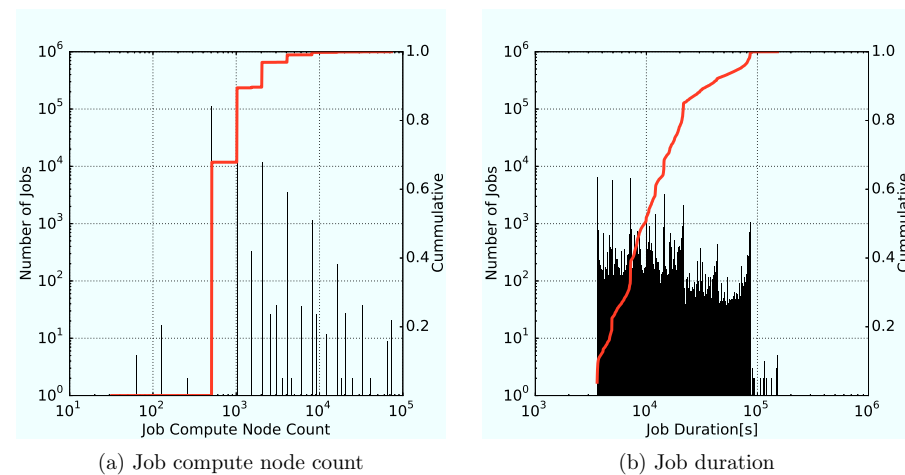
FIGURE 4.10: Histogram and cumulative distribution of job compute node count and job duration
