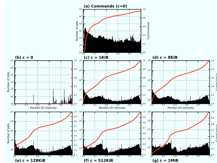
FIGURE 4.32: Parallel I/O intensity for analysed jobs computed using various thresholds c . (a) I/O commands c = 0 , (b) c = 0\text{B} , (c) c = 1\text{KiB} , (d) c = 8\text{KiB} , (e) c = 128\text{KiB} , (f) c = 512\text{KiB} and (g) c = 1\text{MiB} .
