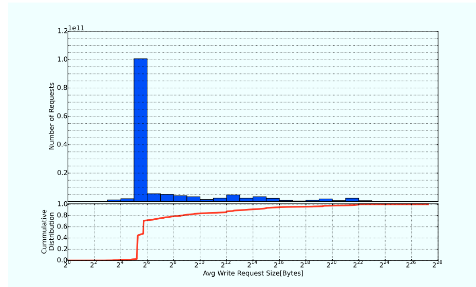
FIGURE 4.25: Distribution of write request sizes.
