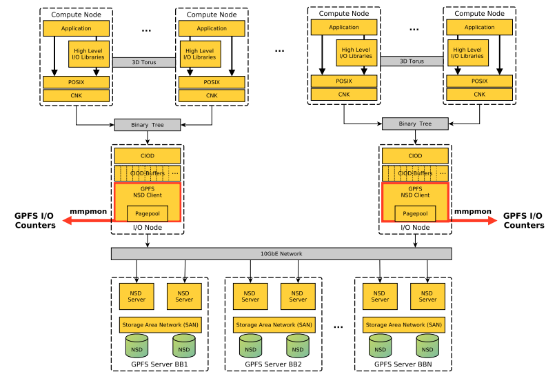
FIGURE 2.3: Location of GPFS I/O counters in JUGENE I/O stack, adapted from [5]
