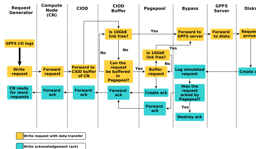
FIGURE 5.3: I/O model write flow graph.
