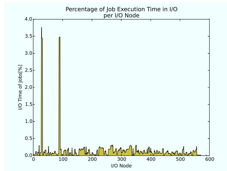
FIGURE 5.9: Simulated percentage of job execution time in I/O for each I/O node.
