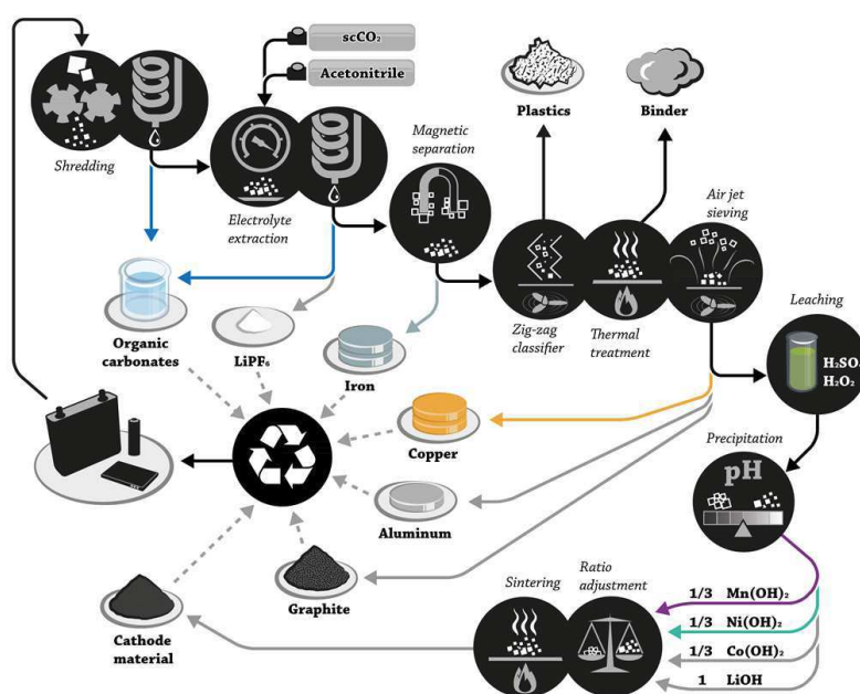
Figure 4. The mechanical-hydrometallurgical “LithoRec II” recycling process. It was reproduced from reference [127], with permission from John Wiley & Sons 2016. \text{scCO}_2 : supercritical carbon dioxide.
