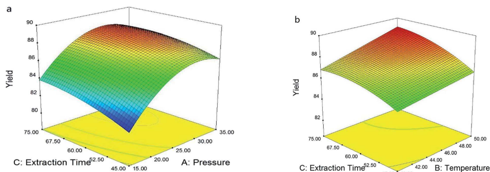
Figure 8. Response surfaces and contour plots for: (a) extraction time vs. pressure; and (b) extraction time vs. temperature. It was reproduced from reference [162] with permission from the Royal Society of Chemistry, 2014.
