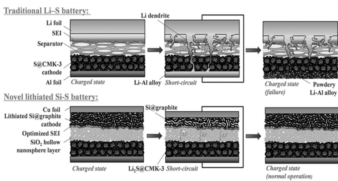
Figure 17. Improved safety of Li-ion/S cells compared to Li/S cells. External short-circuit leading to degradation of the Al current collector in Li/S cells and, therefore, a cell failure. In Li-ion/S cells, no Al current collector degradation took place, enabling the recovery of the cells after abusive conditions. Reproduced with permission from [193] Copyright 2016, Wiley-VCH.
