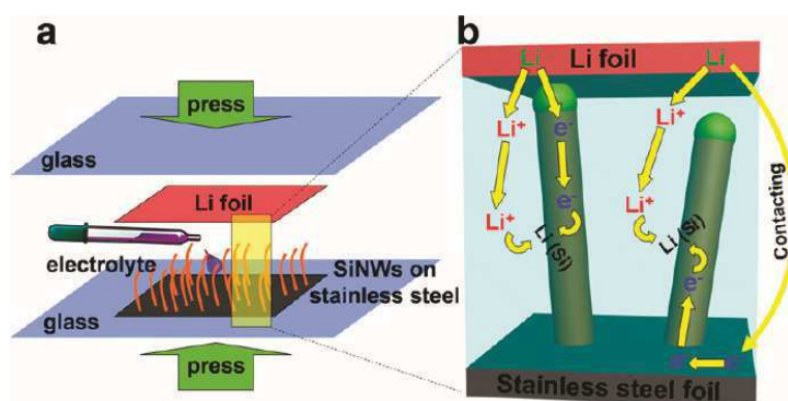
Figure 7. Schematic diagrams showing (a) the pre-lithiation of Si nanowires (SiNWs) on stainless steel foil and (b) the internal electron and \text{Li}^+ pathways during the pre-lithiation. Two possible electron pathways are shown in (b). Electrons can flow directly into the SiNW if the nanowire tip contacts the Li foil, or the electrons can flow across the contacting point of Li foil and stainless-steel foil and enter the SiNW through the bottom. Reproduced with permission from [63] Copyright 2011, American Chemical Society.
