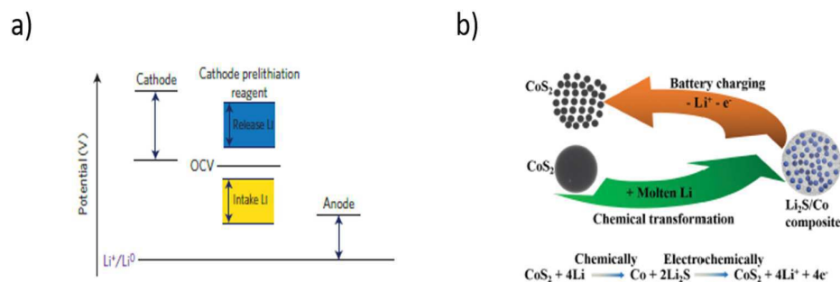
Figure 12. (a) Schematic drawing of the required working potential of the pre-lithiation additive. Reproduced with permission from [114] Copyright 2017, Springer Nature. (b) Synthesis of the Li 2 S/Co additive and the release of the Li + during the initial cycle. Reproduced with permission from [115] Copyright 2017, Wiley-VCH.
