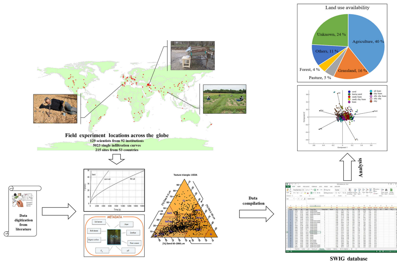
Figure 1. SWIG flowchart.
