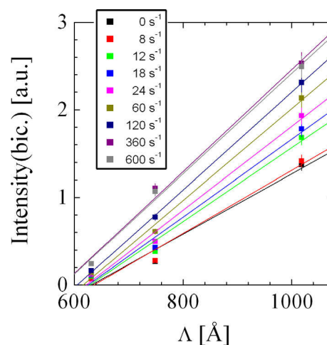
Fig. 6. (color) The intensities of the bicontinuous microemulsion as a function of the scattering depth for different apparent shear rates. (For interpretation of the references to colour in this figure legend, the reader is referred to the web version of this article.)
