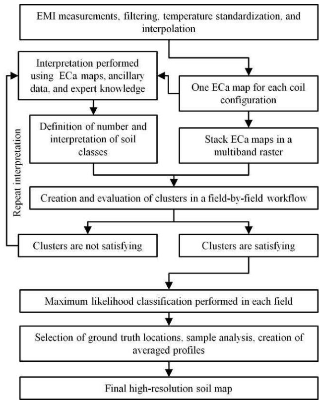
992 Figure 3. Flowchart of the supervised classification methodology.
