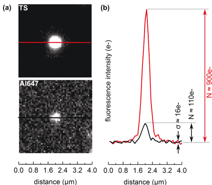
FIGURE 4.3: (a) 4\ \mu\text{m} \times 4\ \mu\text{m} area cutouts of a TS bead and a single Alexa647 dye. The comparison of the intensity profile plots (b) of the bead and the single dye show exemplarily the relation between the noise \sigma and the signal height of a single dye and a TS bead. Typically, the determined SNR are <10 for single dyes and >10 for TS beads.
