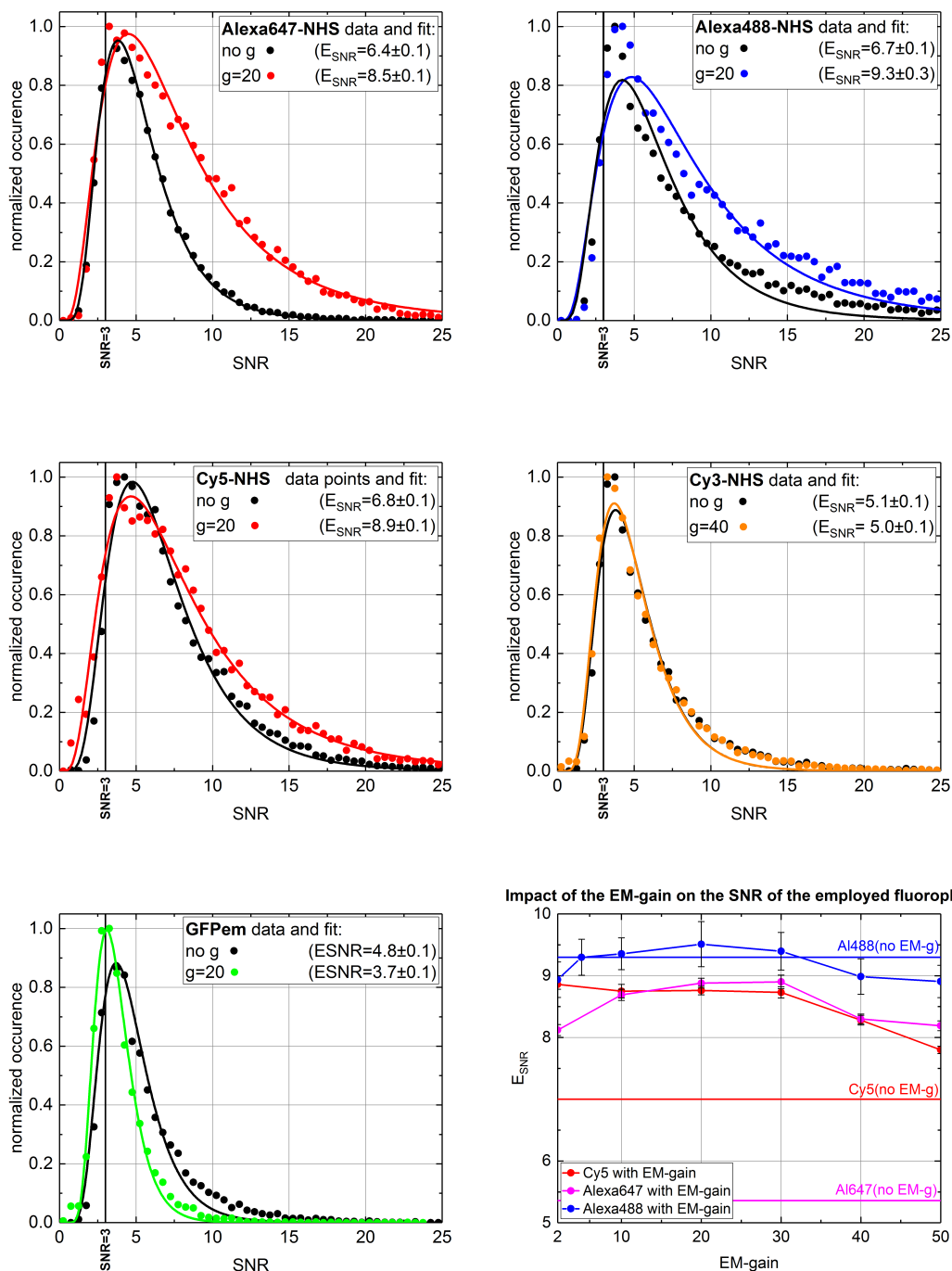
FIGURE 6.11: Impact of the EM-gain on the different fluorescence intensity distributions and E_{\text{SNR}} .
