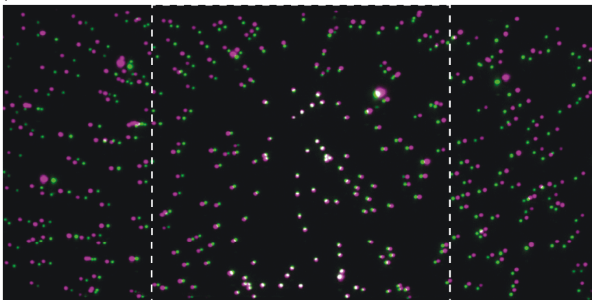
FIGURE 4.12: (a) Illustration of the lateral chromatic aberration, off-axis. (b) Direct red and green channel overlay of an 80\ \mu\text{m} \times 40\ \mu\text{m} area with TS bead positions not corrected for lateral chromatic aberration.
