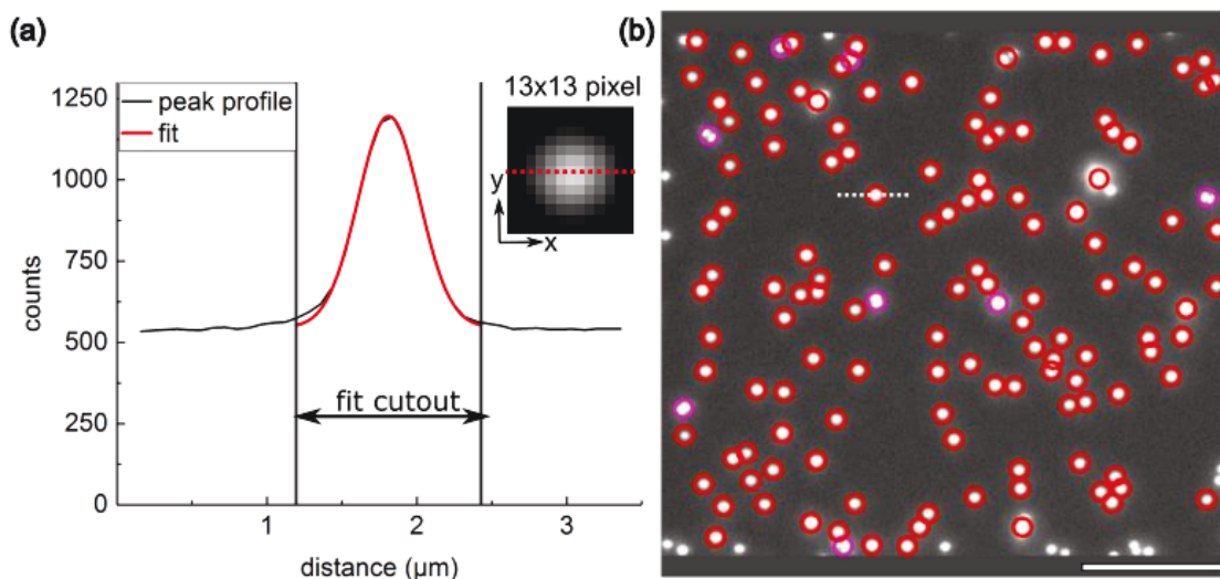
FIGURE 5.4: (a) A profile plot of a TS bead, together with the marked size of the cutout and the Gaussian fit (shown along the x-axis). (b) The figure generated by the routine (scale bar of 10 \mu\text{m} ) with the marked potential peaks and accepted peaks having passed the quality check (red circles).
