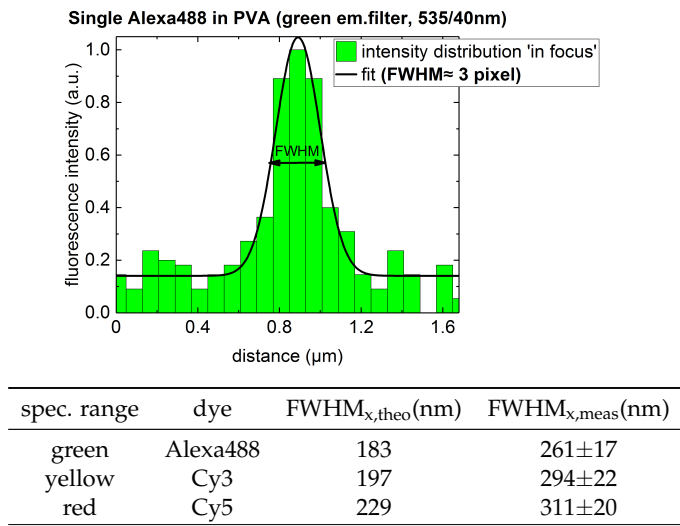
FIGURE 4.11: The determined \text{FWHM}_x derived from the imaging parameter optimization (chapter 6) in the three spectral ranges, together with a representative profile plot of a single Alexa488 dye in the green spectra and the marked \text{FWHM}_x of approximately 3 pixel.
