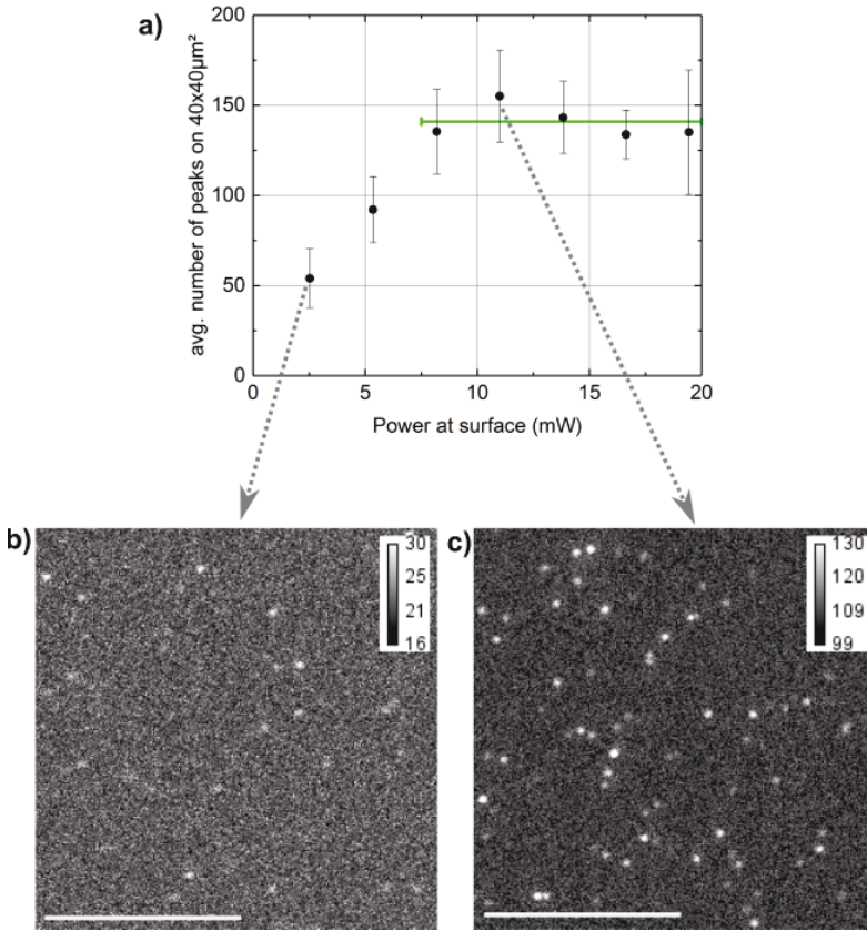
FIGURE 6.7: (a) Excitation power vs. number of identified peaks per image on the example of GFPem. The number of visible peaks increases with power and reaches eventually a plateau, marked with a green bar. Two examples of image sections taken from the GFPem power-series at an excitation power of 2.5mW and 11mW are shown in (b) and (c) respectively, displaying a difference considering the number of visible fluorescence peaks, as well as their SNR (Scale bar of 10 μm, calibration bar in counts).
