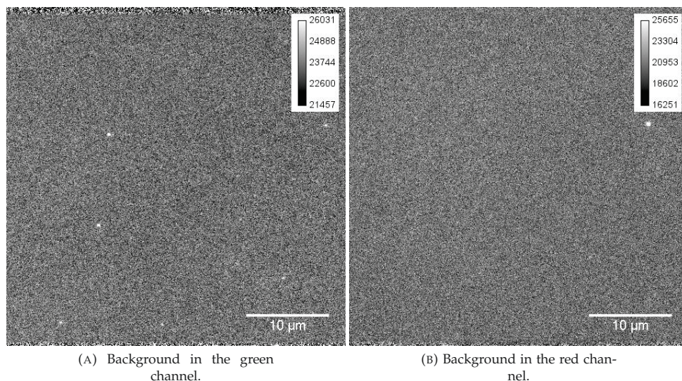
FIGURE 7.3: Representative background images of a 40\text{ }\mu\text{m} \times 40\text{ }\mu\text{m} area in the green (a) and the red channel (b) of a bioPEG surface imaged with Tico buffer.
