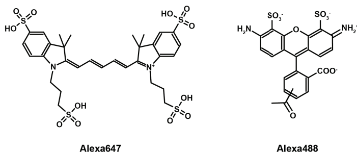
FIGURE 6.2: The chemical structure of the Alexa488 and Alexa647 [90].
