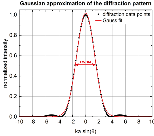
FIGURE 2.4: The profile of the intensity pattern of a diffraction-limited object and the corresponding Gaussian approximation
