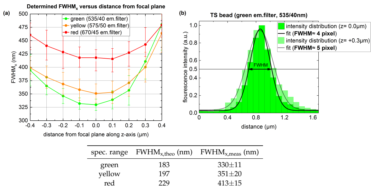
FIGURE 4.10: The \text{FWHM}_x determined from a z-stack of images in the three spectral ranges (a). The error bars correspond to the RMS of the fitted signals. For illustration, representative profile plots along the x-axis of a TS bead are shown, imaged (in the green channel) at the focal plane and 0.3 \mu\text{m} above. In focus, a TS bead displays an FWHM of approximately 4 pixel in the green spectra (b). The table lists the expected \text{FWHM}_{x,\text{theo}} and the measured \text{FWHM}_{x,\text{meas}} in the three spectral ranges. \text{FWHM}_{x,\text{theo}} was calculated according to equation 2.16, taking into account the central wavelength of the auxiliary emission filters (535 nm, 575 nm, 670 nm, see figure A.2 on page 105) and the objective's NA of 1.49.
