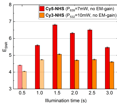
(B) The SNRs' arithmetic means vs. illumination-time for Cy3-NHS and Cy5-NHS. The E_{\text{SNR}} depicted by faint bars were derived from image series recorded with a read out rate of 10 MHz and by applying an EM-gain of 20 (see section 6.3.5).
