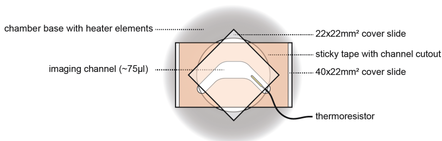
FIGURE 8.5: A sketch of the cover slide sandwich, mounted on top of the heated chamber base. The imaging chamber, with the thermoresistor necessary for the monitoring of the temperature inside the channel, had two openings, that were closed during the time-measurements.
