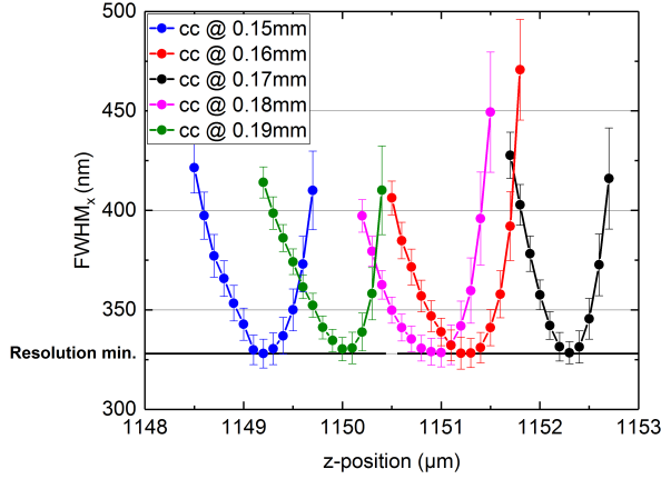
FIGURE 4.9: Impact of the objective's correction collar on the \text{FWHM}_x of TS beads on the surface
