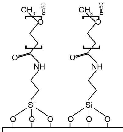
FIGURE 7.1: The surface protocol steps
