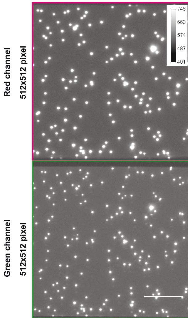
FIGURE 5.1: The two color channels of the central 40\ \mu\text{m} \times 40\ \mu\text{m} section of a TS bead image, displaying in each color approximately 120 TS signal peaks (scale bar 10\ \mu\text{m} ).
