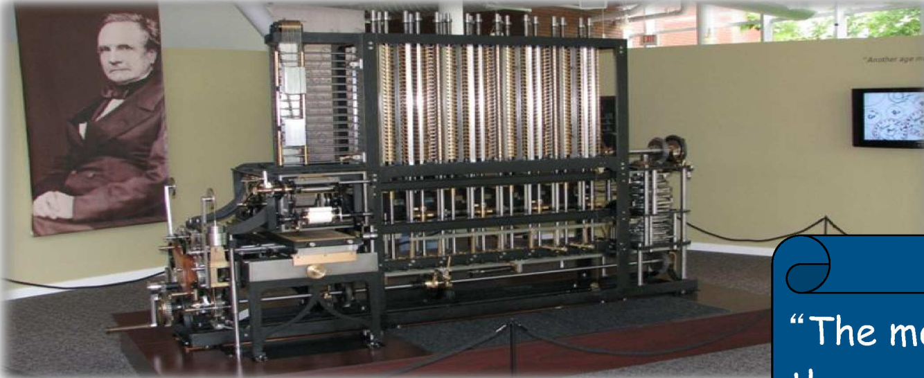
Difference Engine
