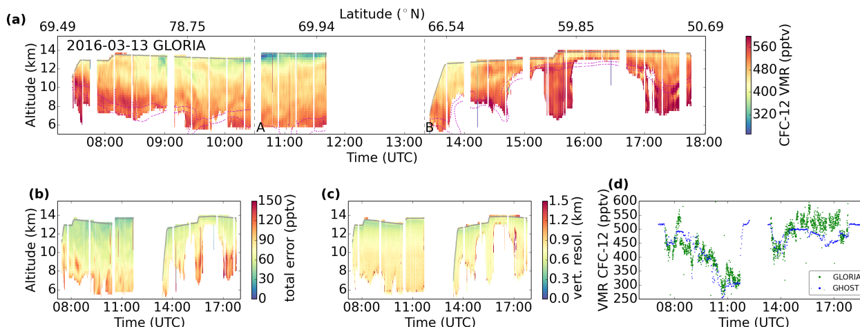
Figure 11. CFC-12 flight PGS19: Cross section of (a) retrieved CFC-12 volume mixing ratio (the flight altitude is marked with a grey line, the ECMWF potential vorticities of 2 and 4 PVU are marked with magenta dashed lines, way points are marked with grey vertical dashed lines). Cross sections of (b) total estimated error, (c) vertical resolution and (d) comparison of the GLORIA measurements (green) to the GhOST-MS in-situ measurement (blue).
