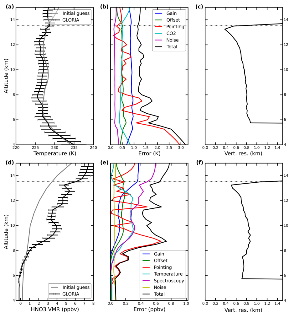
Figure 4. Illustration of the error budget of the temperature and \text{HNO}_3 retrieval of flight 19 on 13 March 2016 for a selected profile at 10:37:06 UTC. (a, d) retrieved vertical profile of temperature (a–c) and \text{HNO}_3 (d–f) with total estimated error (black) and initial-guess profile (gray). The retrieved profile has 14.9 and 12.5° of freedom for temperature and \text{HNO}_3 , respectively. (b, e) Different total error contributions and estimated total error. (c, f) Vertical resolution of this retrieval result. The dotted line represents the flight altitude of the aircraft.
