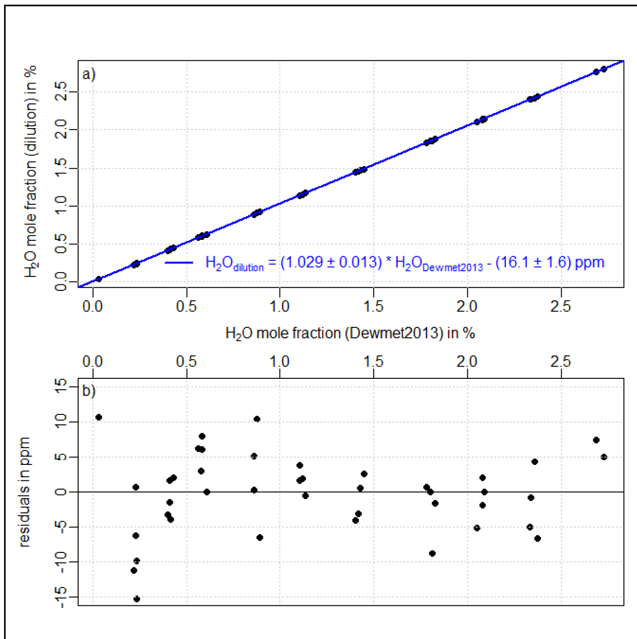
Figure 6: a) Water vapor mole fraction based on the CO 2 dilution method plotted against the water vapor mole fraction measurement of the CRDS analyzer (offset corrected and calibrated according to the comparison against a dew point mirror in 2013) during the fine scan experiment. The corresponding fit is shown in blue. Residuals (difference between water vapor mole fraction based on dilution method and the linear fit) can be seen in plot (b).
