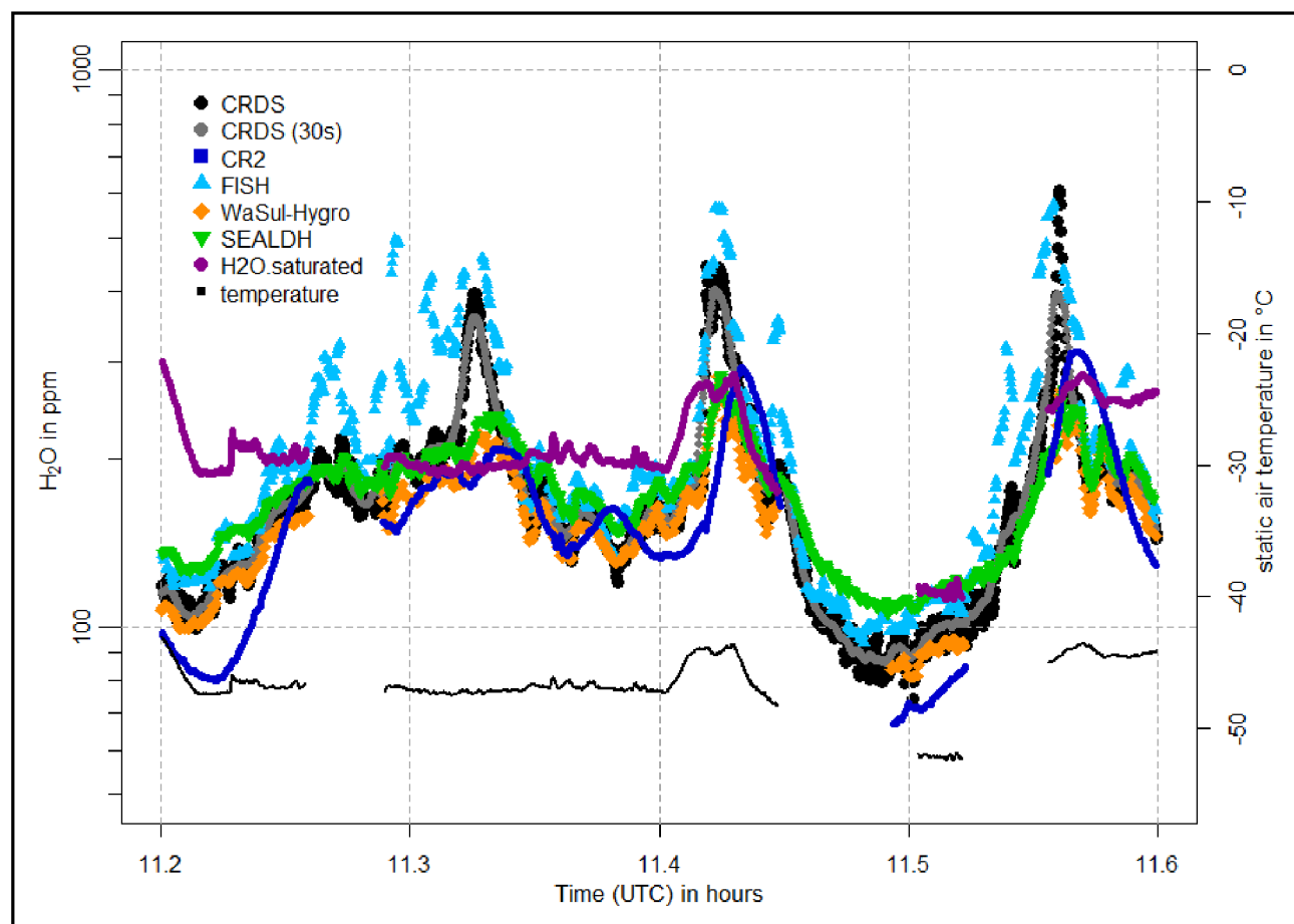
Figure 12: Water vapor mole fractions of the CRDS analyzer (offset corrected and calibrated according to the 2013 dew point mirror comparison) (black points, 30 seconds mean as grey points), the CR-2 (dark blue squares) and FISH (light blue triangles) instruments, as well as the WaSul-Hygro (orange diamonds) and SEALDH-I (green triangles) analyzers, during the flight on 1 June 2011, in the presence of clouds. Also shown are the water vapor mole fraction corresponding to saturation (violet points) and the static air temperature (black line).
