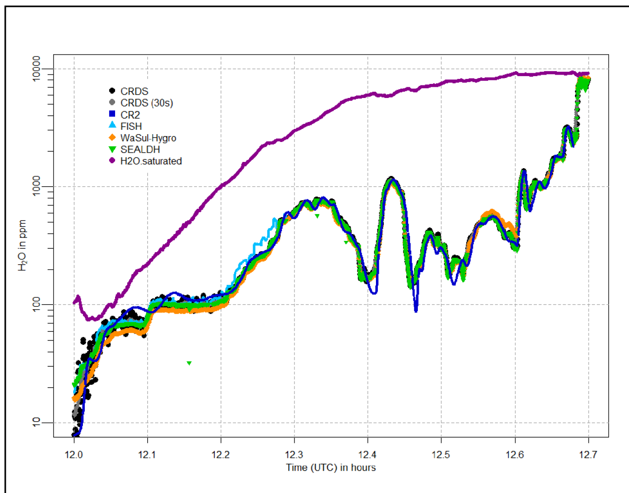
Figure 9: Same as Fig. 8, but for a time period during the flight on 1 June 2011.
