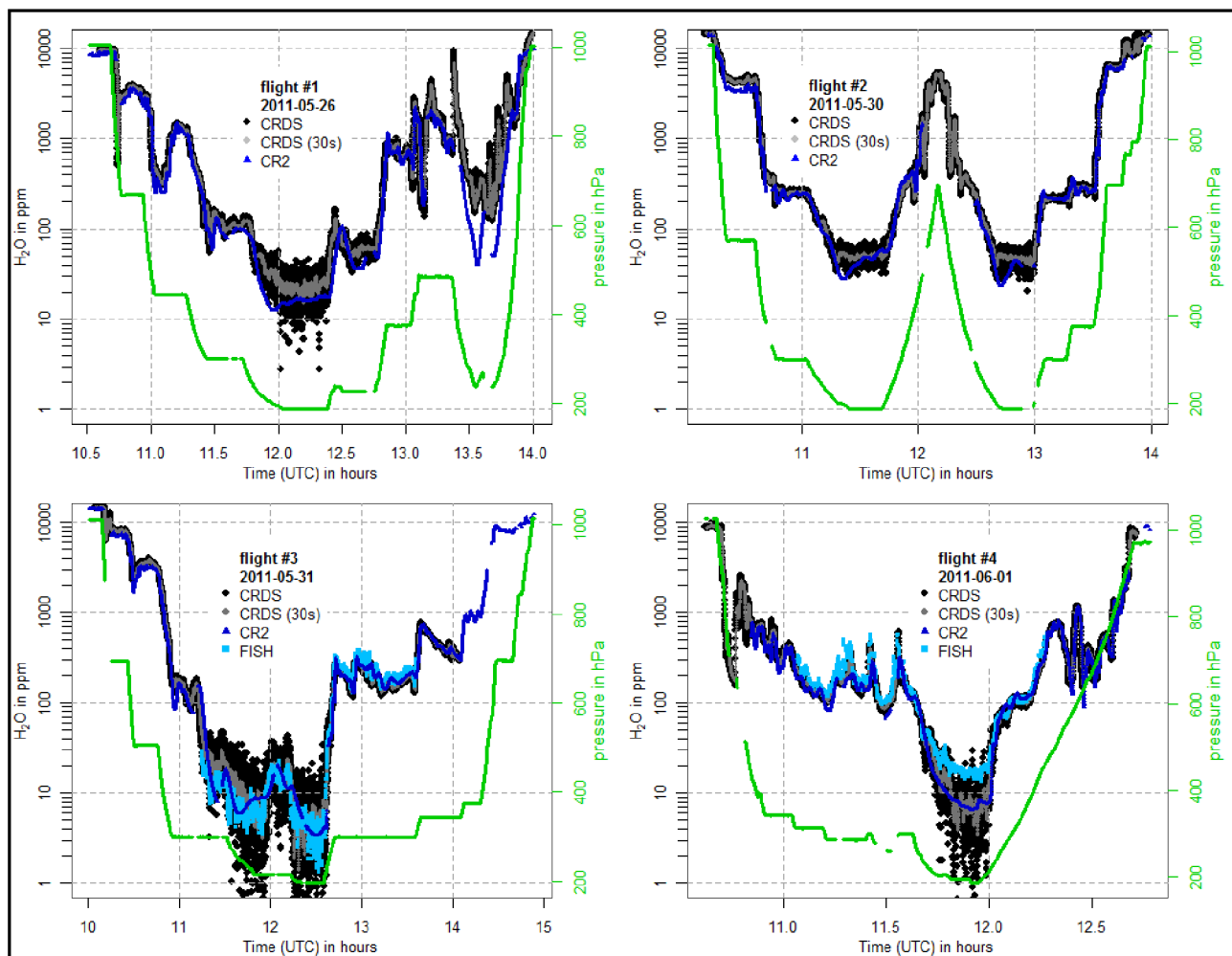
Figure 10: In-flight water vapor data of the CRDS analyzer (in black, 30 seconds mean in grey) and the reference instruments CR-2 (in dark blue) and FISH (in light blue) for the four flights on 26 May, 30 May, 31 May, and 1 June 2011. The corresponding atmospheric pressure levels are shown in green. The CRDS data are offset corrected and calibrated according to the 2013 dew point mirror comparison.
