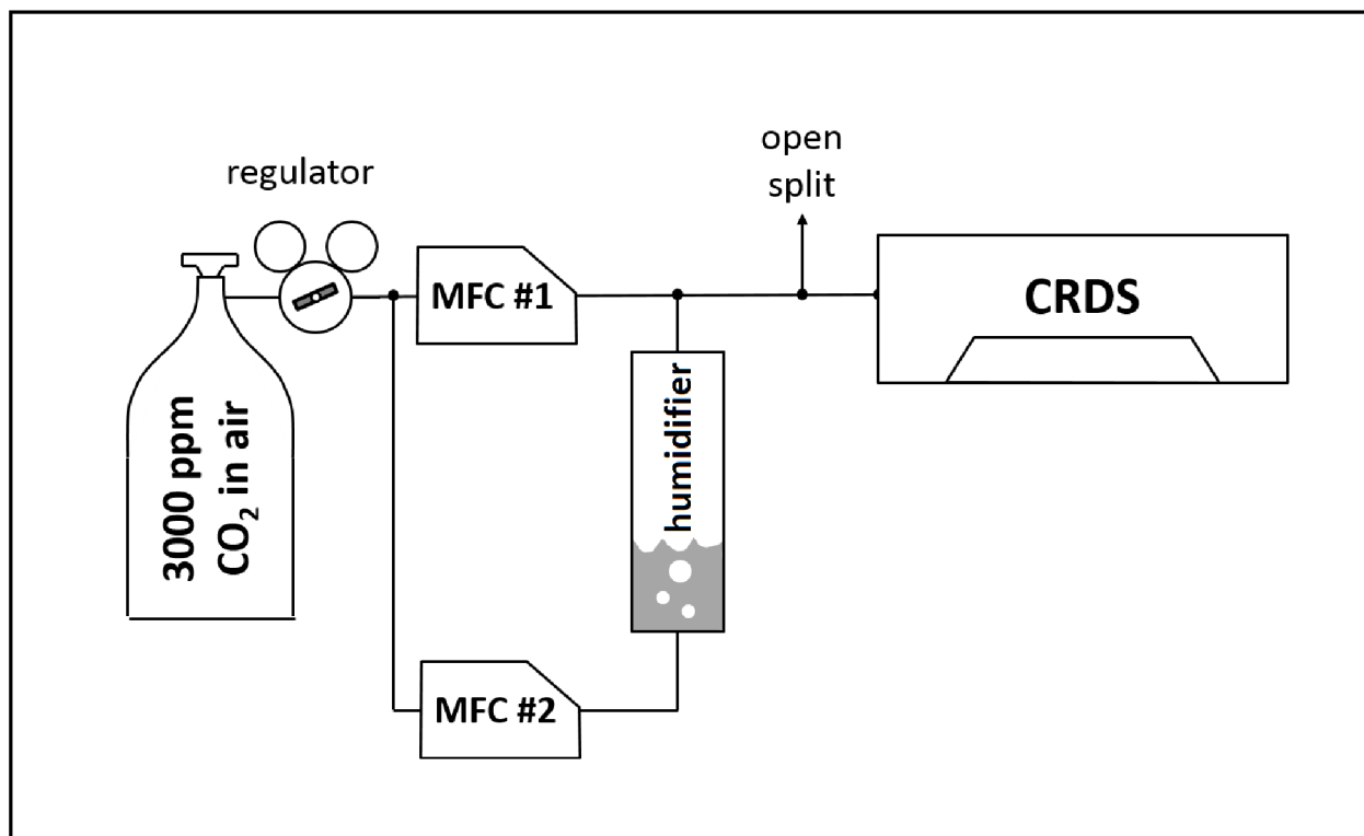
Figure 2: Experimental setup for the water vapor calibration by the CO 2 dilution effect.
