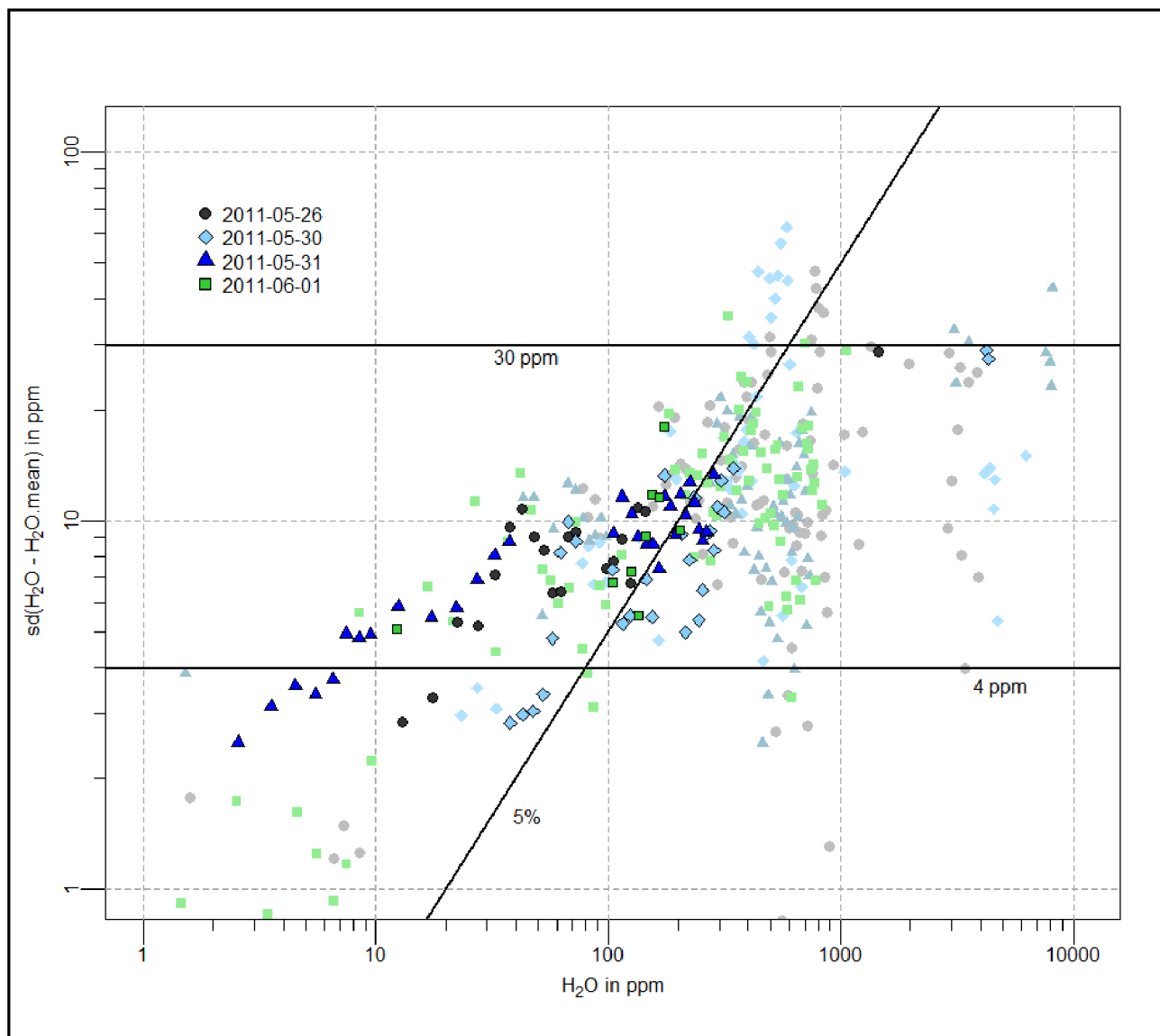
Figure 7: Standard deviation of the difference between the 0.4 Hz data (offset corrected and calibrated according to the 2013 dew point mirror comparison) and the 60 second averages, averaged for intervals of 1 ppm, 5 ppm, 10 ppm, and 100 ppm water vapor in the corresponding water vapor ranges of 0-10 ppm, 10-100 ppm, 100-1000 ppm, 1000-10000 ppm, respectively. Different colors and symbols indicate different flights. Results with higher priority are highlighted. The horizontal and diagonal black lines indicate standard deviations of 4 ppm, 30 ppm, and 5 % (rel.) respectively.
