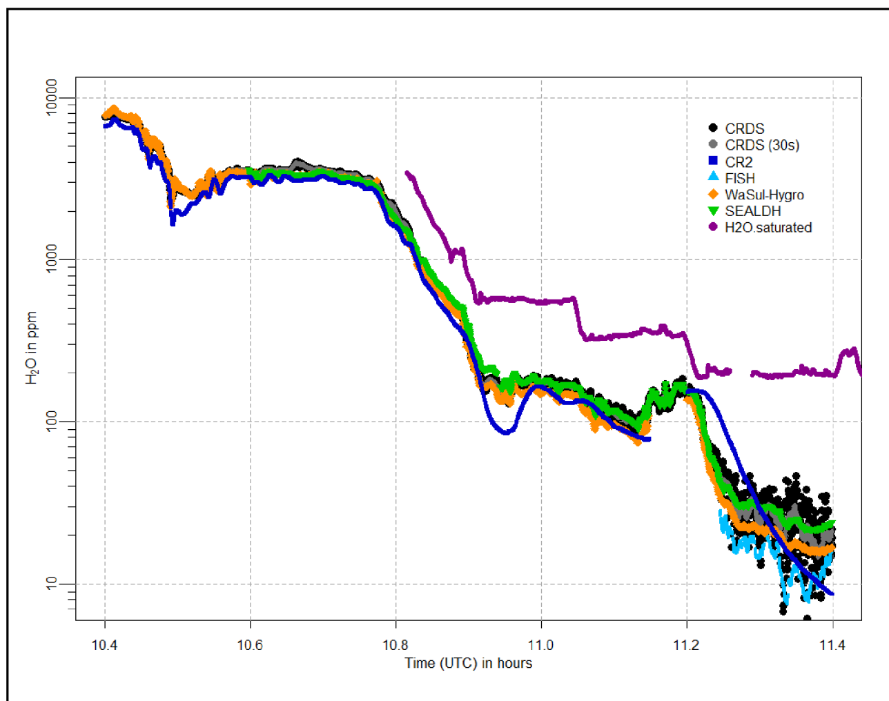
Figure 8: Water vapor mole fractions of the CRDS analyzer (offset corrected and calibrated according to the 2013 dew point mirror comparison) (black points, 30 seconds mean as grey points), the CR-2 (dark blue squares) and FISH (light blue triangles) instruments, as well as the WaSul-Hygro (orange diamonds) and SEALDH-I (green triangles) analyzers, for a time period during the flight on 31 May 2011.
