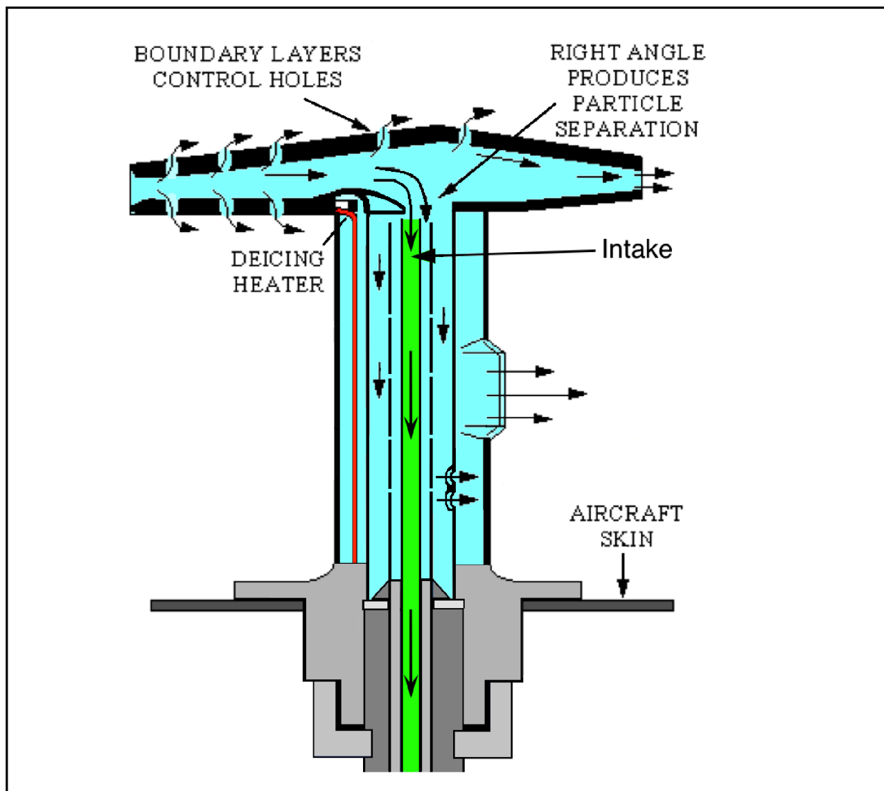
Figure 1: Cross section of the inlet line (green) mounted into a Rosemount Total Air Temperature housing (model 102B, adapted from Stickney et al. (1994)). The inlet line is pointed orthogonal to the airflow through the housing to prevent from sampling larger aerosols, ice particles, and water droplets.
