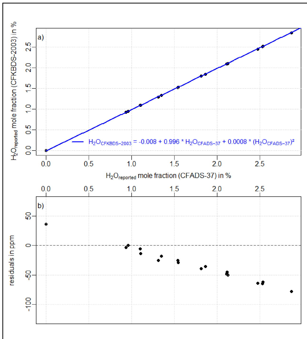
Figure 4: a) Uncalibrated water vapor mole fractions of the two Picarro CRDS analyzers CFADS37 and CFKBDS2003 during a comparison experiment in 2014 (black points). The blue line indicates the quadratic fit of an earlier comparison between the same instruments in 2011. The differences between the two comparisons, thus the drift of the two analyzers over the three years from 2011 to 2014, are shown in plot (b).
