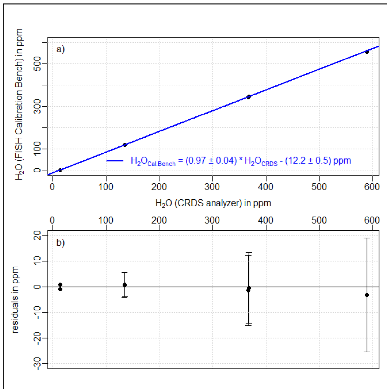
Figure 5: a) Dry air water vapor mole fractions measured by the CFKB2004 CRDS analyzer and the FISH calibration bench during a comparison in 2011. The CRDS data are calibrated according to the 2013 comparison against a dew point mirror. The corresponding fit is shown in blue. Residuals (difference between water vapor mole fractions measured by FISH calibration bench and the linear fit) can be seen in the plot (b). Error bars indicate the uncertainty range of the calibration bench of 4 % (rel.).
