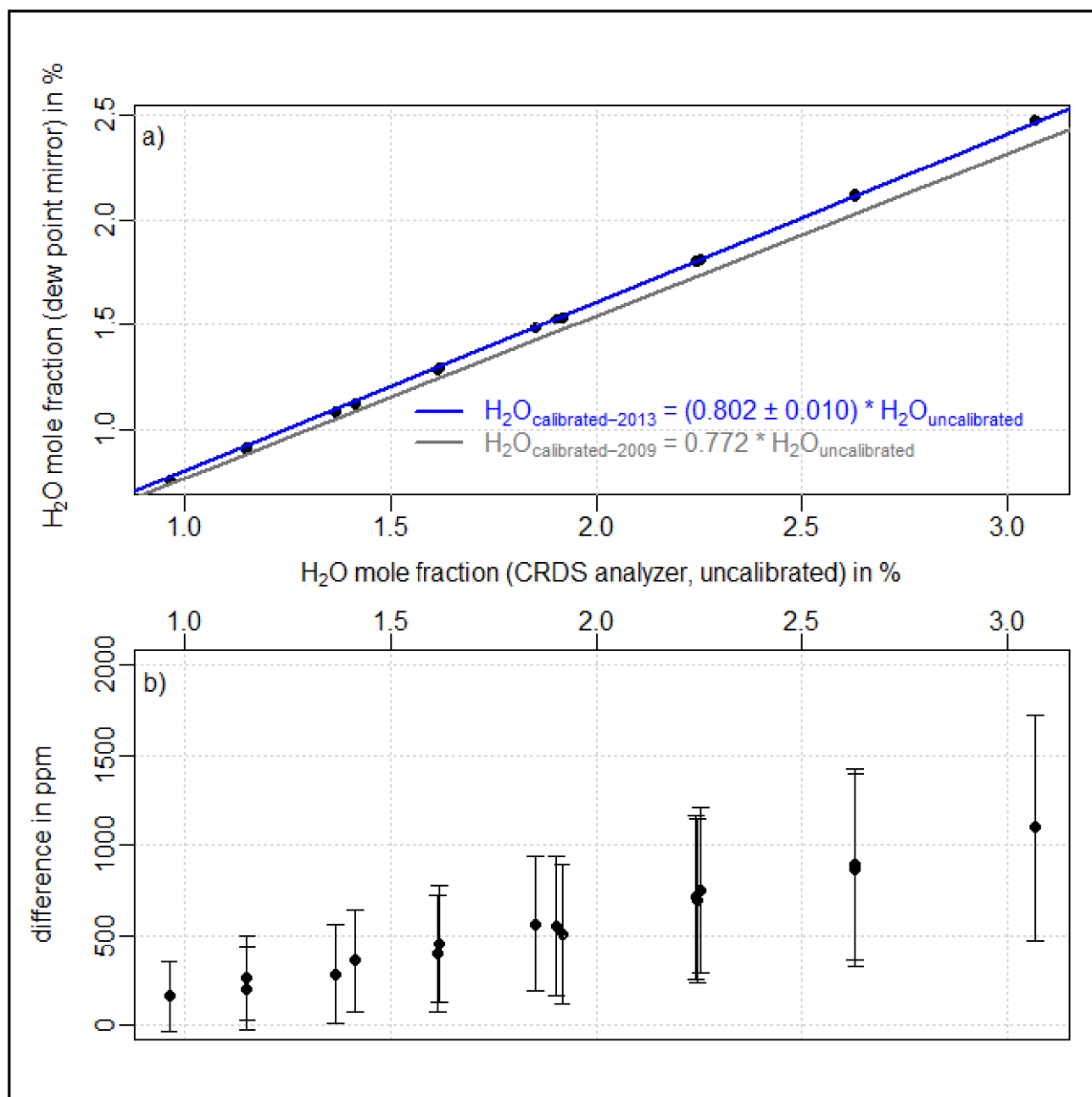
Figure 3: a) Uncalibrated water vapor measurements of the Picarro CRDS analyzer (CFKBDS2003) against the measurements of the dew point mirror (Dewmet TDH) during the 2013 calibration. The corresponding fit is shown as blue line, the calibration curve of the 2009 comparison as a grey line. The uncertainty of the fitted slope is composed of the fitting error and the uncertainty of the dew point mirror. b) Water vapor difference between the 2009 and 2013 experiments. The error bars indicate the uncertainty range, which results from the combination of the dew point mirror uncertainties during the 2009 and the 2013 calibration.
