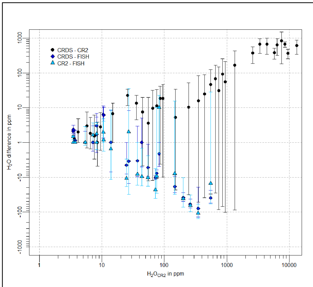
Figure 11: Absolute differences of the 30 seconds mean CRDS and CR-2 in-flight data (black points), CRDS and FISH data (dark blue diamonds), and CR-2 and FISH data (light blue triangles) averaged over intervals of 1 ppm, 10 ppm, 100 ppm, 1000 ppm, and 10000 ppm water vapor in the corresponding water vapor ranges of 0-10 ppm, 10-100 ppm, 100-1000 ppm, 1000-10000 ppm, and >10000 ppm, respectively, against the CR-2 water vapor flight data. Error bars indicate the standard deviations of the average differences.
