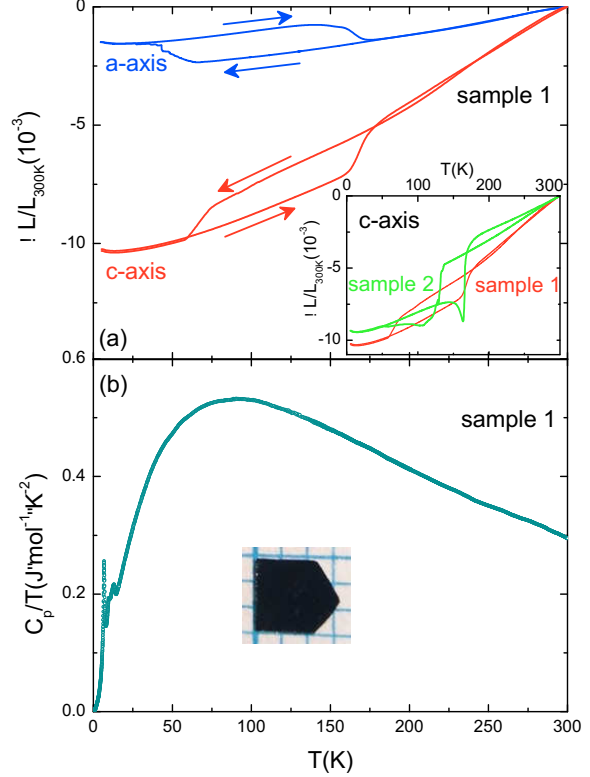
FIG. 1. (a) Temperature dependence of the thermal-expansion of \alpha -RuCl 3 along a (blue curves) and c (red curves) axes. A structural transition with a huge hysteresis is observed in both directions (arrow down: cooling, arrow up: heating). Inset: The hysteresis of the structural transition of a second sample (sample 2) is considerably smaller. (b) Specific heat versus temperature (upon cooling) clearly showing anomalies at the magnetic transition, however no clear anomalies at the structural transition. A photograph of Sample 1 is shown in the inset.
