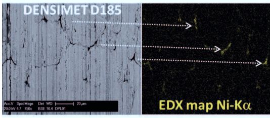
Figure 1: SEM image and EDX map of the DENSIMET D185 surface (machined, as received).
