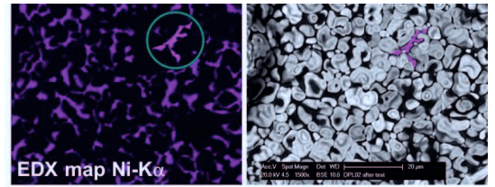
Figure 6: SEM image and EDX map of the HPM1850 tile surface after the high heat flux test in GLADIS with surface temperatures \leq 2200^\circ\text{C} ( 20 \text{ MWm}^{-2} , 3 s).
