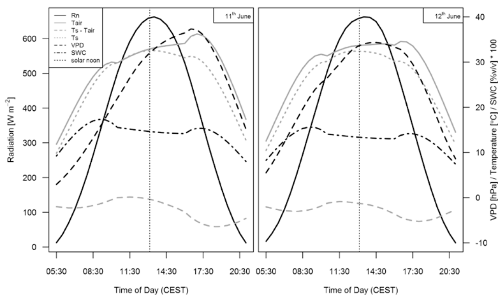
Figure 2. Environmental conditions (net radiation ( R_n ), air temperature ( T_{air} ), surface temperature ( T_s ), T_s - T_{air} , vapour pressure deficit (VPD), as well as soil water content (SWC)) for 11th and 12th of June 2014 over a non-treated grass surface measured by the weather station.
