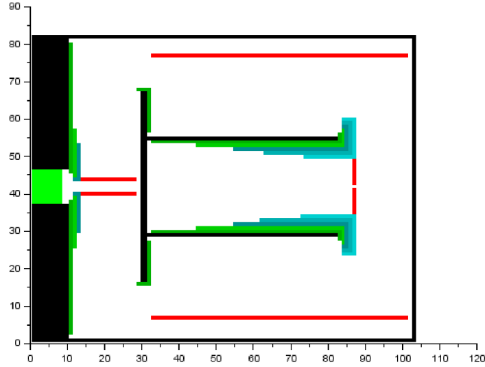
Fig. 4. Lanes (green/blue) and shifted inner convergence line (red)
