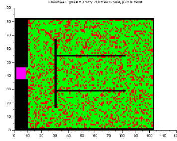
Fig. 1. Starting positions for all simulations. The size of the floor is 83 by 102 cells of 40 \times 40 \text{ cm}^2
