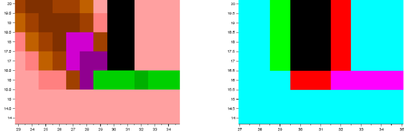
Fig. 3. left: Utilization of tiles at corner of wall (black) without conflicts , from pink-low (0-25) to dark green – high (>600), right: divergence (green) and convergence (red/purple) lines.
