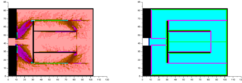
Fig. 2. left: Utilization of tiles without conflicts (persons near exit start first, others wait till persons in front are out of reach), from pink–low(0-25) to green–high(>400) right: Exit (blue), walls (black) divergence lines (green) and convergence lines (purple)
