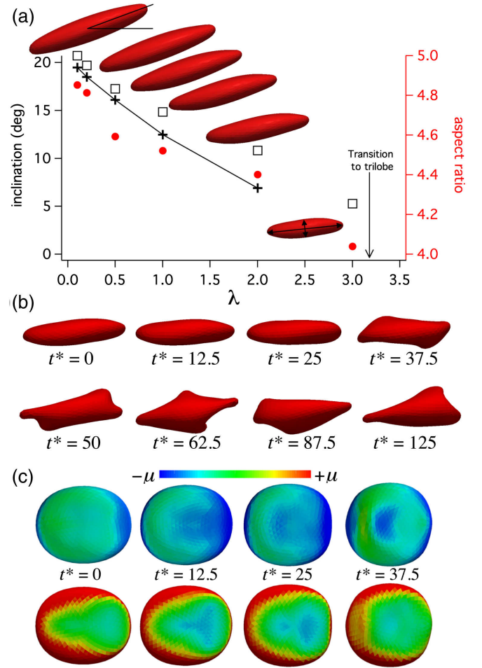
FIG. 4. Trilobe formation. (a) Inclination angle (square and plus symbols, left axis) and aspect ratio (maximum to minimum size, red circles, right axis) of a RBC as a function of \lambda at \dot{\gamma}^* = 1.36 from YALES2BIO simulations. The square and bullet symbols correspond to simulation measurements, while the plus symbols are obtained from the Keller-Skalak theory for fluid vesicles [41] using cell dimensions measured in simulations. (b) Time evolution ( t^* = \dot{\gamma}t ) of shapes at \lambda = 3.5 (starting from a simulation with \lambda = 3.1 ), when TT becomes unstable and a trilobe is formed (see movie S6). (c) Membrane's elastic tension in the direction of the smallest (top) and largest (bottom) local strains.
