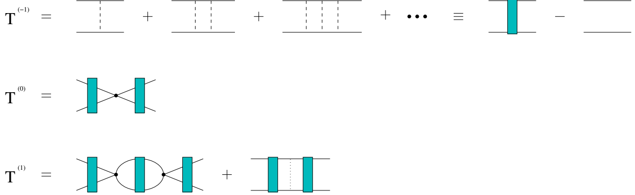
FIG. 1: Leading, next-to-leading and next-to-next-to-leading order contributions to the scattering amplitude in the KSW-like approach. The solid lines denote nucleons while the dashed ones represent an insertion of the lowest-order long-range interaction. Solid dots (dotted lines) denote an insertion of the lowest-order contact interaction \propto C_0 (subleading contribution to the long-range interaction).
