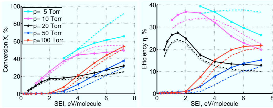
Figure 2: Results of 1D calculations with self-consistent electron density and gas temperature
