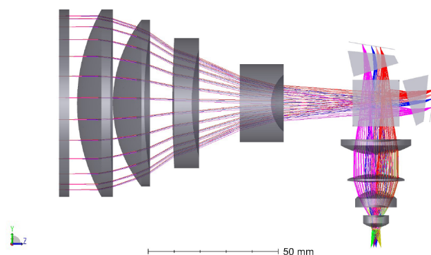
Figure 5. Optical components of the instrument, including the interference filter, the front optics, the SHS, the detector optics, and the detector.
