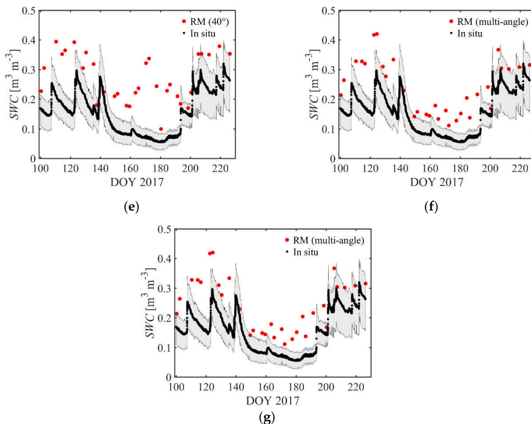
Figure 11. Volumetric soil water content (SWC) [ \text{m}^3 \text{m}^{-3} ] retrieved from T_B observations over the non-gridded plot using different retrieval schemes (see Table 1) with the \tau - \omega model. Inversions were performed using either the single-angle approach ( 40^\circ incidence angle) (a,c,e) or the multi-angle approach (from 40^\circ to 60^\circ incidence angle) (b,d,f,g). The retrieval schemes depicted here are, namely, the 1-P retrieval scheme (a,b), the 2.1-P retrieval scheme (c,d), the 2.2-P retrieval scheme (e,f), and the 3-P retrieval scheme (g). The estimated SWC values are compared to the in situ measured SWC in 5 cm depth. The grey shaded areas represent the 75% quintile of the in situ sensors.
