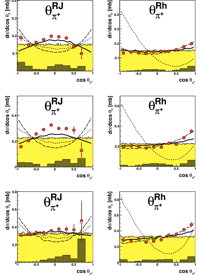
FIG. 12: (Color online) Same as Fig. 5, but for the angles of positive pions in the D_{21} resonance subsystem either in the Jackson frame ( \theta_{\pi^+}^{RJ} , left) or in the helicity frame ( \theta_{\pi^+}^{Rh} , right) for the energy bins at T_p = 1.10 (top), 1.18 (middle) and 1.31 GeV (bottom).
