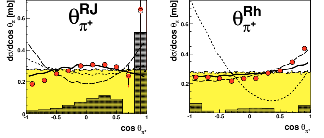
FIG. 7: (Color online) The same as Fig. 6, but for the angles of positive pions in the D_{21} resonance subsystem either in the Jackson frame ( \Theta_{\pi^+}^{R,J} , left) or in the helicity frame ( \Theta_{\pi^+}^{R,h} , right).
