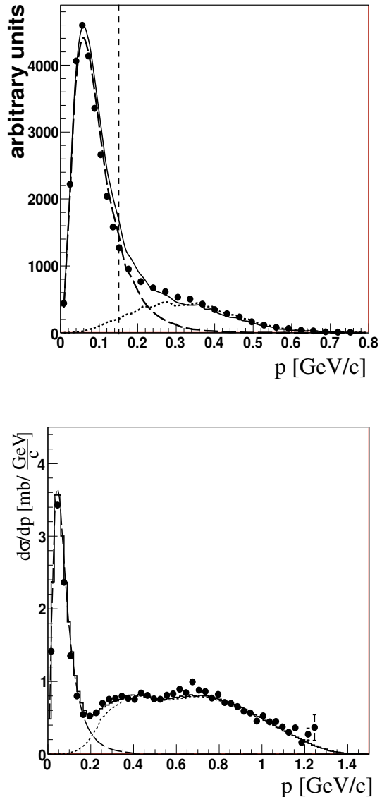
FIG. 1: (Color online) Distribution of the neutron momenta in the pd \rightarrow pp\pi^+\pi^- reaction before (top) and after acceptance and efficiency correction (bottom). Data are given by solid dots. The dashed line shows the expected distribution for the quasifree process pd \rightarrow pp\pi^+\pi^- + n_{spectator} based on the CD Bonn potential [42] deuteron wavefunction. The vertical line indicates the region p < 0.15 GeV/c used for the evaluation of the quasifree process. The dotted line gives the modeling of the non-quasifree reaction process. The solid line is the incoherent sum of both processes.
