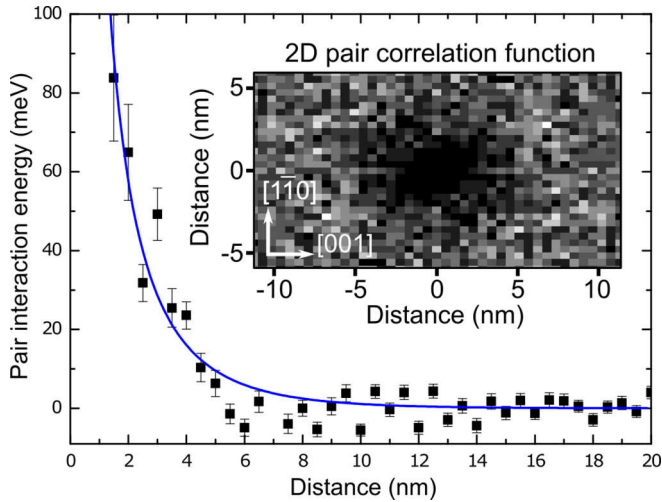
FIG. 12. Radial pair interaction energy derived from the pair-correlation function (inset) deduced from the spatial position of the antisites in STM images. The solid blue line is a fit of a three-dimensional bulk screened Coulomb potential model near the growth surface (i.e., with surface dielectric constant, see text). The data points to a +1e charged state of the antisites during incorporation at the (001) growth surface.
