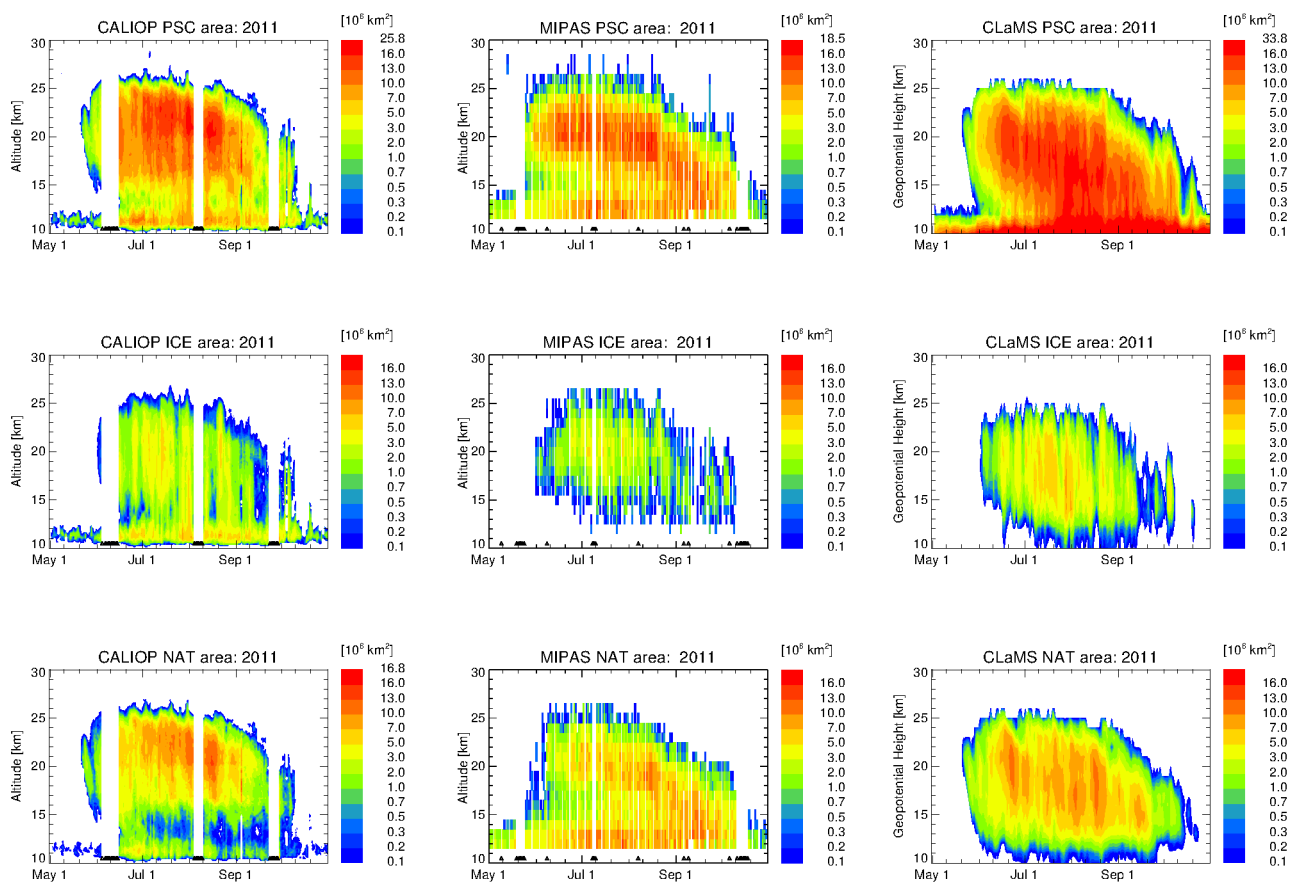
Figure 6. Same as Fig. 2 but for the 2011 SH winter from 01 May 2011 until 31 October 2011. Here, MIPAS observations and CLaMS simulations are restricted to latitudes < 82^\circ \text{ S} .
