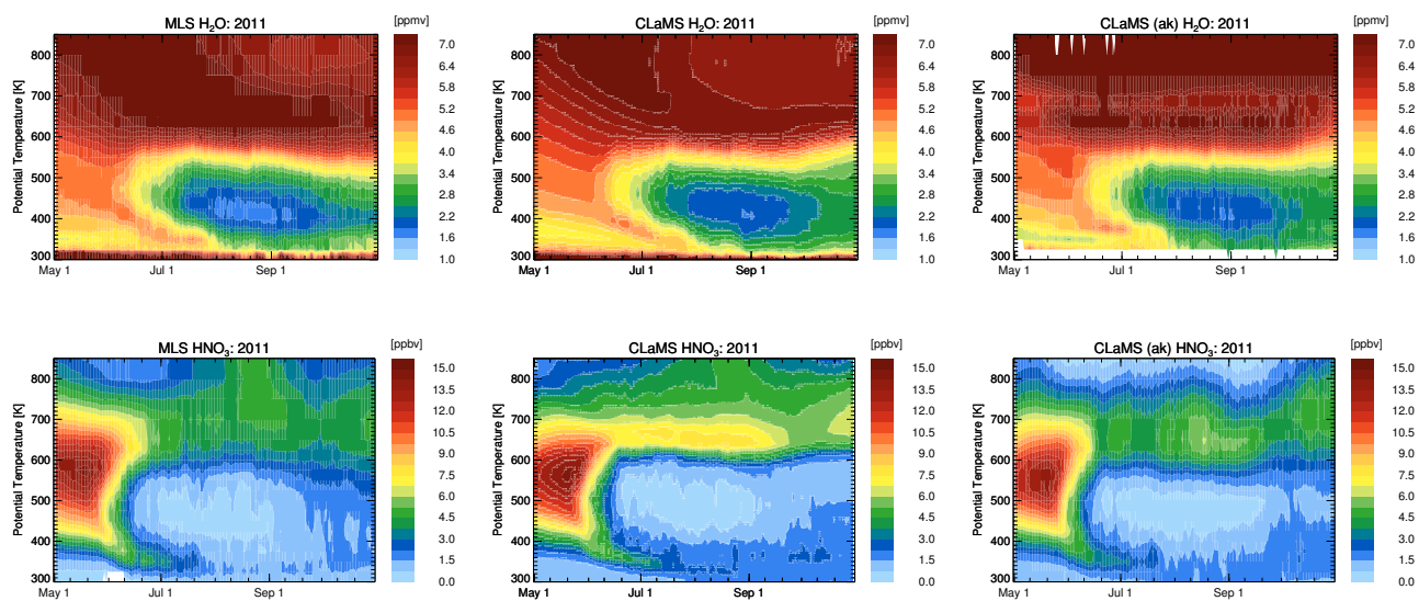
Figure 10. Same as Fig. 5 but for the 2011 SH winter from 01 May 2011 until 31 October 2011 and for equivalent latitudes > 70^\circ S.
