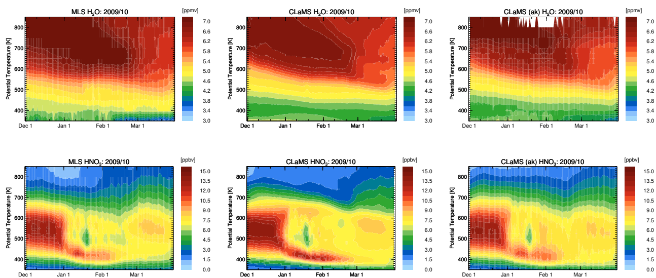
Figure 5. Temporal evolution of water vapor ( \text{H}_2\text{O} , top row) and nitric acid ( \text{HNO}_3 , bottom row) are shown as an average inside the core of the polar vortex (equivalent latitudes > 70^\circ \text{N} ) from 01 December 2009 until 31 March 2010. MLS measurements are presented in the left column, CLaMS model results in the middle column and CLaMS model results accounting for the MLS averaging kernel in the right column.
