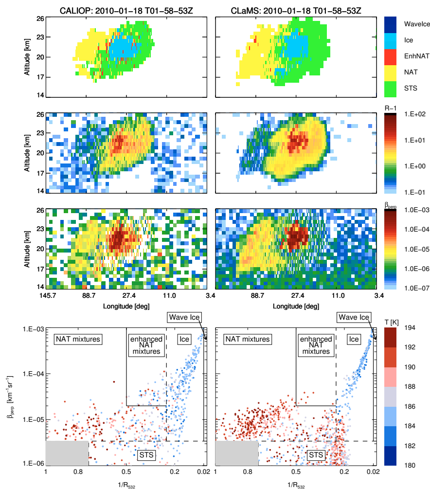
Figure 3. 18 January 2010: CALIPSO orbit track 2010-01-18T01-58-53Z. CALIOP measurements are shown in the left column, corresponding model results in the right column. First row: CALIOP PSC classification v2; second row: aerosol backscatter ratio ( R - 1 ); third row: perpendicular backscatter signal ( \beta_{\text{perp}} ); lowermost row: inverse backscatter ratio ( 1/R ) vs. perpendicular backscatter signal ( \beta_{\text{perp}} ) with data color-coded by temperatures taken from GEOS-5 and ERA-Interim for CALIOP and CLaMS, respectively, and overlaid CALIOP v2 PSC composition classification scheme.
