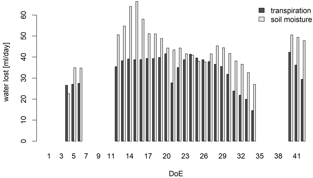
Figure A.5: Comparison of daily sums of transpired water to water loss calculated with the variations in soil moisture content. Time spans when water was added to the column were excluded.
