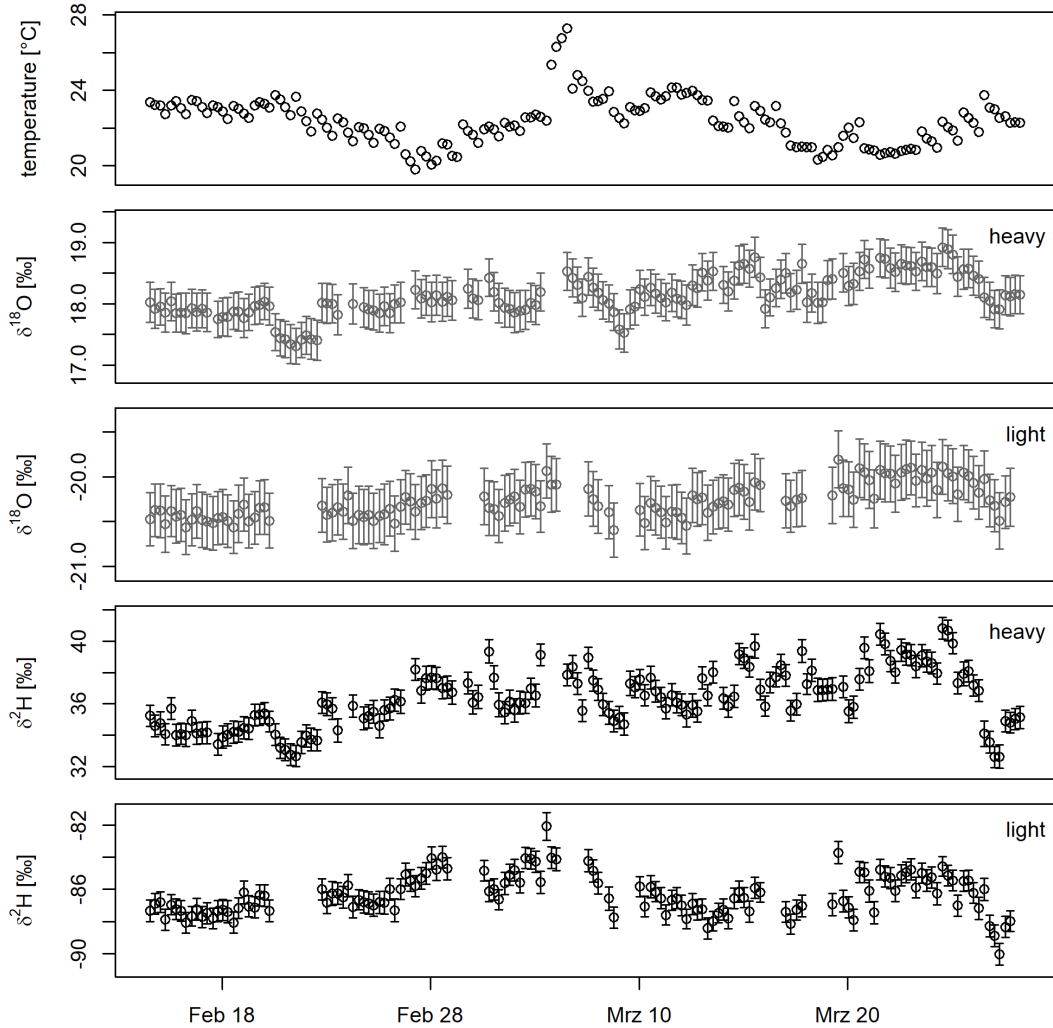
Figure 4.6: Timeline of processed and sorted measurements for St_{light} and St_{heavy} and the temperature measured in the insulated standard box. Isotopic compositions are reported as mean values with their respective standard deviations.
