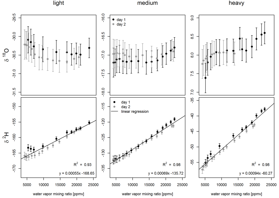
Figure A.2: Instrument specific dependency between isotope ratios and water vapor mixing ratio of the sample gas. Linear regressions used for correcting measurements of \delta^2\text{H} are also plotted with their equation and R^2 .
