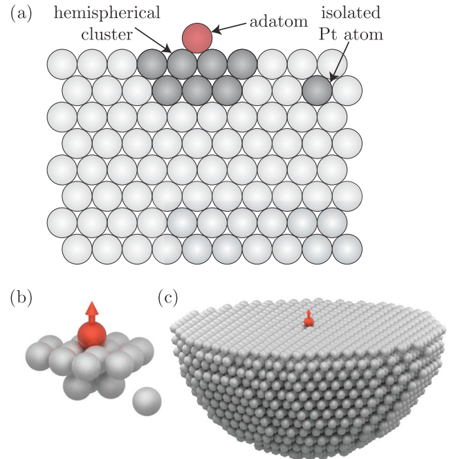
FIG. 4. Illustration of the cluster used for the giant hemispherical calculations. (a) The adatom (red sphere) is embedded on an arbitrary surface (light and dark gray spheres). The cluster used for each small calculation contains a hemisphere around the adatom (dark gray spheres) and one additional isolated host atom (dark gray sphere). (b) Three-dimensional visualization of the Pt(111) cluster used here. (c) Total giant hemispherical cluster containing 2685 Pt atoms, which is used for the calculation of the interatomic orbital moment.
