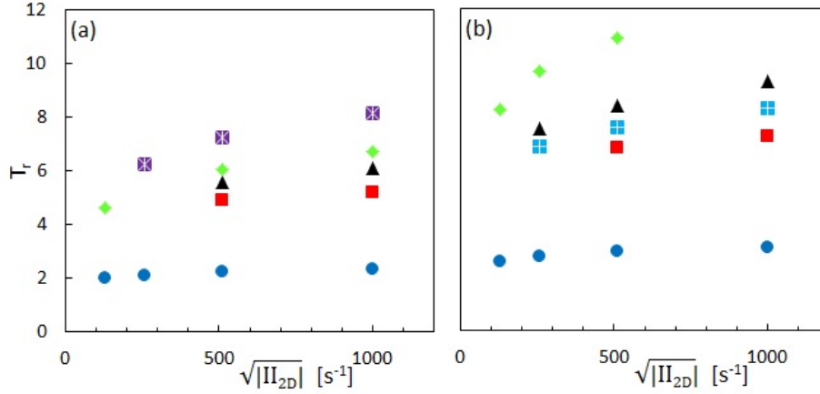
Figure 10. Trouton ratio as a function of the square root of the second invariant of the rate of deformation tensor for different concentrations of (a) fd and (b) fdY21M. Legend, see figure 7.
