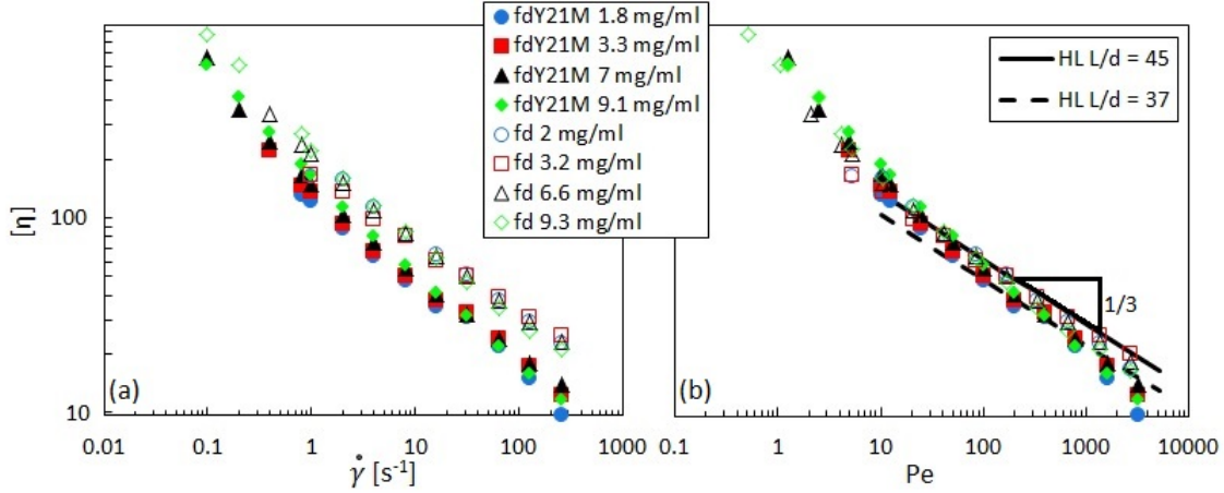
Figure 8. (a): Intrinsic viscosity as a function of shear rate for different concentrations. (b): Intrinsic viscosity as a function of Péclet number as defined by equation 2. The line shows a prediction by HL theory.
