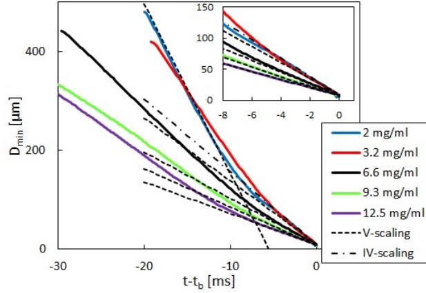
Figure 4. Filament diameter versus time for different concentrations of fd virus. Dashed lines indicate the visco-capillary (V) scaling and dash-dotted lines indicate the inertia-viscous (IV) scaling. Inset: Filament diameter versus time in the terminal region.
