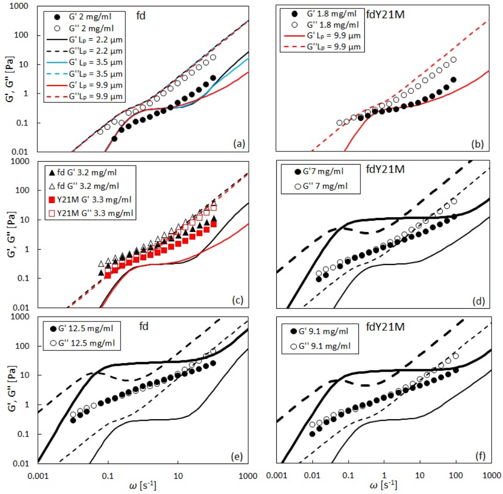
Figure 5. Complex moduli G' (full symbols, full lines) and G'' (open symbols, dashed lines) as a function of frequency for different concentrations of (a), (e): fd; (b), (d), (f): fdY21M and (c) both viruses. The lines are predictions from Morse theory in the dilute (thin lines) and concentrated (thick lines) regime. Numbers in the caption of (a) and (b) indicate different theoretical persistence lengths. For the rest of the figure persistence lengths of 2.2 \mu\text{m} for fd and 9.9 \mu\text{m} for fdY21M are used.
