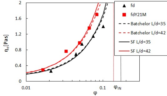
Figure 9. Elongational viscosity of fd (black triangles) and fdY21M (red squares) as a function of concentration. The curves are predictions from Shaqfeh and Fredrickson (SF) and Batchelor theory, using the indicated aspect ratios. The vertical lines mark the position of \varphi_{IN} for both systems.
