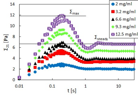
Figure 3. Shear stress as a function of time for different concentrations of fd virus at a shear rate of 10 \text{ s}^{-1} . The horizontal lines mark the stress level at the overshoot \Sigma_{\max} and in the steady state \Sigma_{\text{steady}} for a concentration of 12.5 mg/ml.
