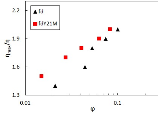
Figure 11. Overshoot viscosity divided by steady state viscosity as a function of concentration at \dot{\gamma} = 10 \text{ s}^{-1} .
