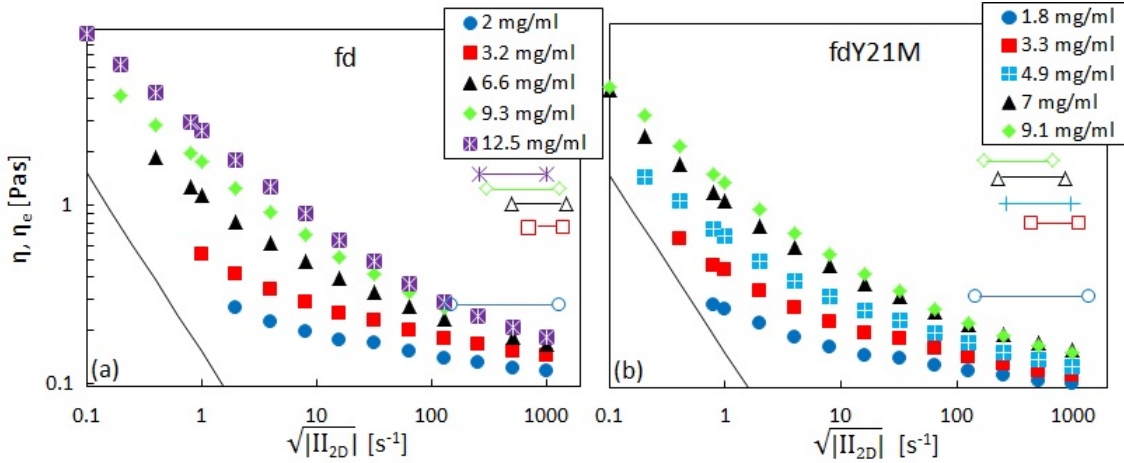
Figure 7. Shear (full symbols) and elongational viscosity (open symbols), as a function of the square root of the second invariant of the rate of deformation tensor for (a): fd and (b): fd Y21M at different concentrations. The thin line marks the lower torque limit of the rheometer.
