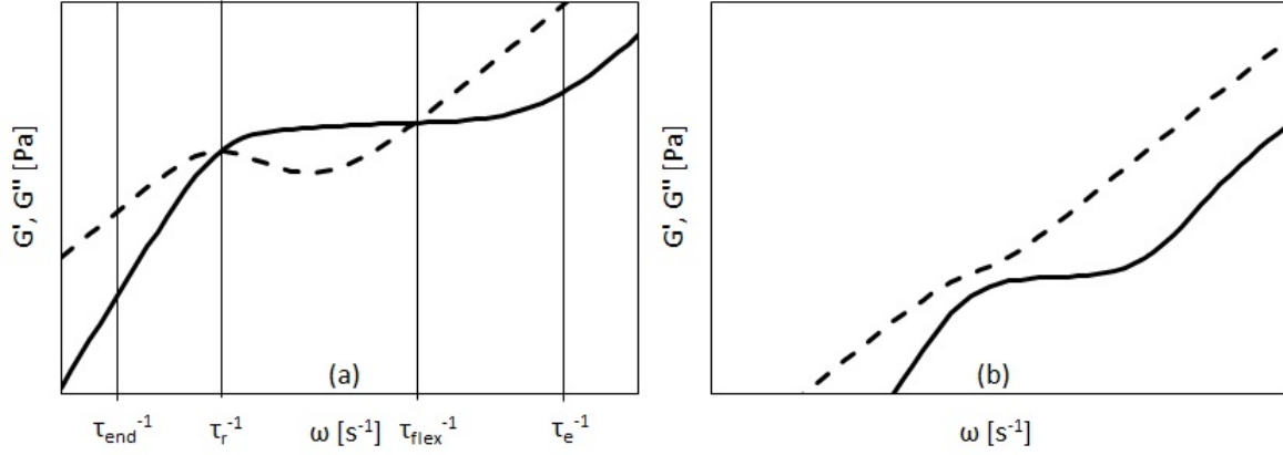
Figure 2. Storage and loss modulus vs. angular frequency from Morse theory for L_p \gg L in the semi-dilute (a) and dilute case (b). Vertical lines in (a) indicate the location of the most important relaxation times.
