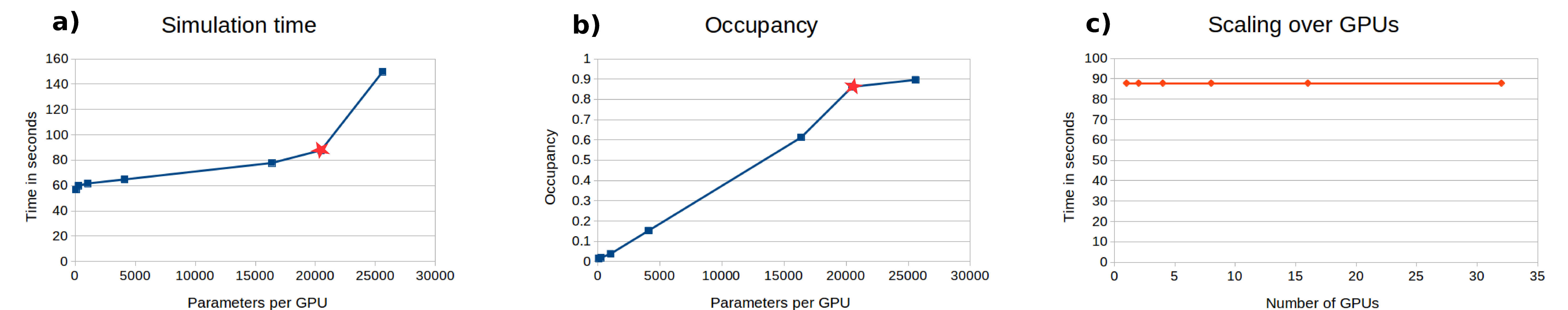
Figure 2: Performance of the CUDA code using the Kuramoto model with changing global coupling and connection speed. a) Simulation time of executing different numbers of parallel simulations on a single GPU. b) GPU occupancy with increasing number of parallel simulations. c) Scaling over different numbers of GPUs with 21600 parallel simulations each. Runs performed on the Jureca cluster (GPU partition) of the Jülich Supercomputing Centre
