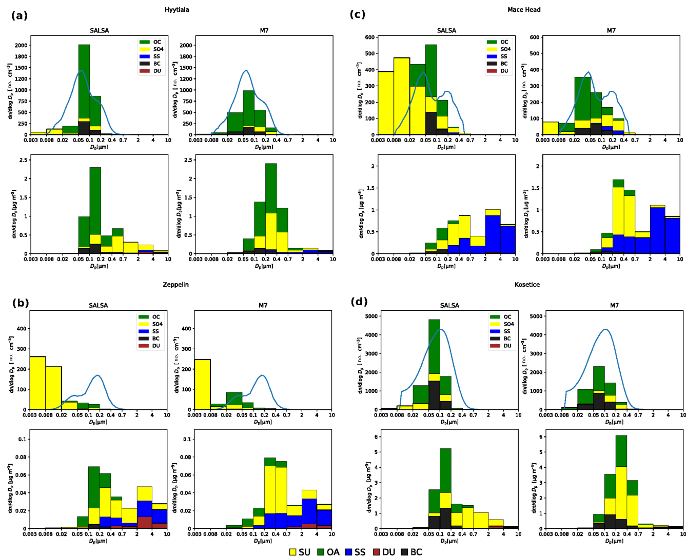
Figure 15. Observed and modeled yearly median number size distributions ( dn/d\log D_p ), and modeled mass ( dm/d\log D_p ) size distributions, for four different EUSAAR stations: (a) Hyytiälä, (b) Mace Head, (c) Zeppelin, and (d) Kosetice. Observed values are represented by the solid blue curves and the modeled are represented by the bar plots. The relative mass contribution of individual chemical compounds in each size class are denoted by a color.
