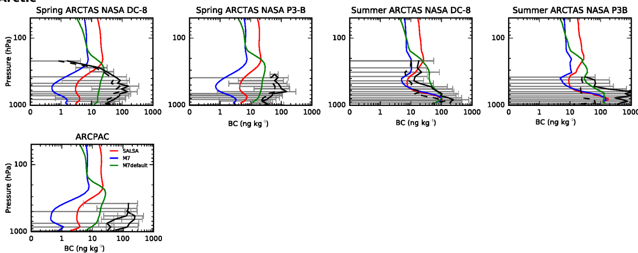
Figure 12. Observed and modeled mean vertical profiles of BC in aircraft measurement campaigns. Black curves represent the measured BC concentrations and the gray whiskers show the variability in measurements.
