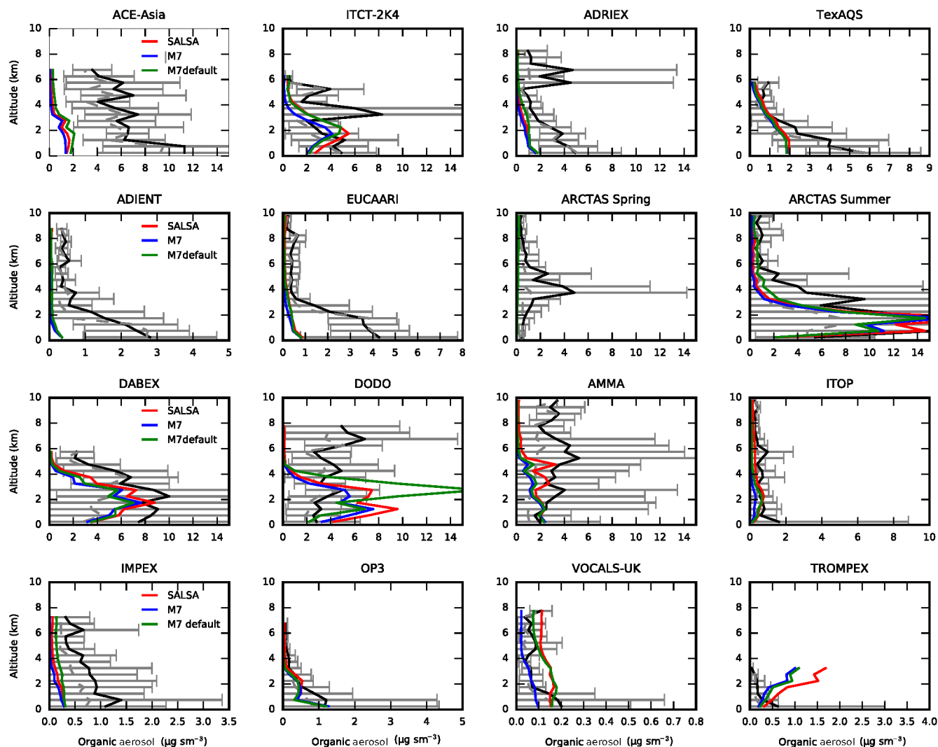
Figure 14. Observed and modeled mean vertical profiles of organic aerosol (OA) in aircraft measurement campaigns. Black curves represent the measured OA concentrations and the gray whiskers show the variability in measurements.
