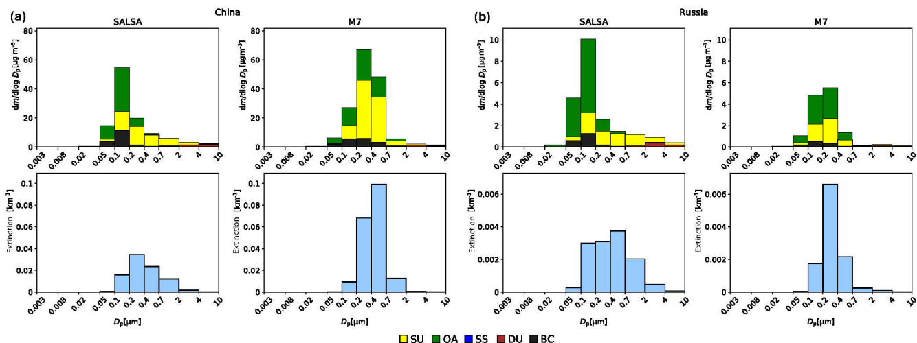
Figure 4. SALSA2.0 and M7 simulated mass ( dn/d\log D_p ) and extinction size distribution in (a) China ( 30.775^\circ N, 114.375^\circ E) and (b) Russia ( 55.025^\circ N, 39.375^\circ E). The height of the bars in the upper row represents the number concentration of particles dN/d\log D_p . The color bars represent the mass fraction of each chemical compound in each size class. In the bottom row the height of the bars denotes the extinction of the size classes.
