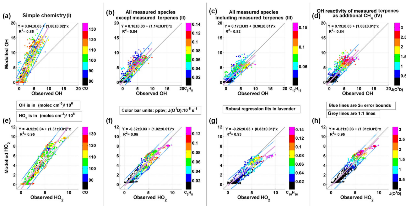
Figure 3. LIF-FAGE measurements of OH (a–d) and HO 2 (e–h) vs. model simulations with CAABA/MECCA. From left to right: model simulations using simple chemistry without NMHCs (case I), simulations including anthropogenic and biogenic hydrocarbons except terpenes (case II), after adding terpenes (case III), and after initializing with zero terpenes but with CH 4 increased to account for the additional measured terpene reactivity (case IV).
