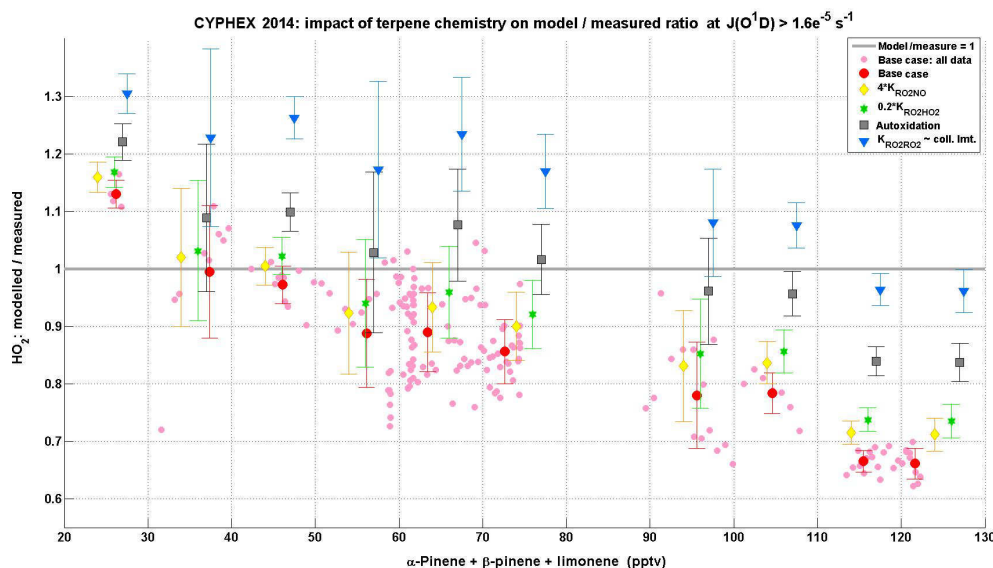
Figure 6. \text{HO}_2 predictions using different chemical schemes which were employed to investigate the impact of peroxy radicals as a \text{HO}_2 sink. The x axis shows the sum of measured \alpha -pinene, \beta -pinene, and limonene. The base case is the model simulation using measured species; 4 \times K_{\text{RO}_2\text{NO}} is a simulation in which the rates of selected terpene-related \text{RO}_2 species with NO are increased by a factor of 4; 0.2 \times K_{\text{RO}_2\text{HO}_2} is a simulation in which the rates of these \text{RO}_2 species with \text{HO}_2 are reduced by a factor of 0.2; the autoxidation simulation includes an autoxidation scheme rapidly converting selected \text{RO}_2 species into ROOH. The last scheme refers to a simulation in which K_{\text{RO}_2\text{R}'\text{O}_2} is set to 4 \times 10^{-10} \text{ cm}^3 \text{ molecule}^{-1} \text{ s}^{-1} (close to the collision limit). The mean and sigma are calculated for 100 pptv bins along the x axis.
