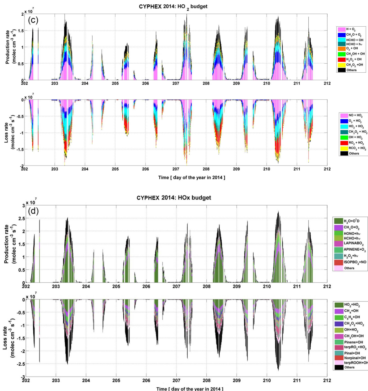
Figure 7. (c) Budget analysis for \text{HO}_2 and (d) budget analysis for \text{HO}_x , during CYPHEX. The descriptions for pinene, \text{terpRO}_2 , and \text{terpROOH} are the same as in Fig. 5.
