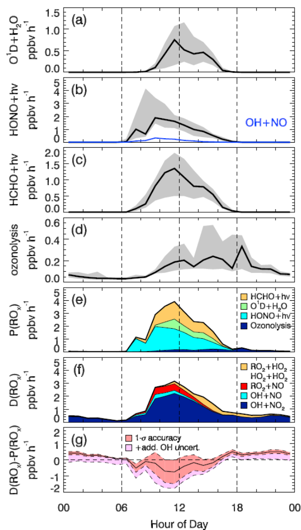
Figure 2 Median production and destruction rates of RO_x . Panels (a - d) show production rates (black lines: median values) from the photolysis of ozone (a), HONO (b), HCHO (c), and ozonolysis of alkenes (d). Grey bands around the median denote 25 % and 75 % percentiles. The blue line in panel (b) represents the back reaction rate of OH+NO yielding HONO. Panels (e) and (f) show cumulative plots of the production and destruction rates, respectively. Panel (g): the solid black line is the difference between the total production and destruction rate. The red shaded band indicates the 1\sigma uncertainty due to experimental errors of the measured quantities (Table S1) and the reaction rate coefficients. The pink shaded area represents the maximum possible bias from a potential OH interference.
