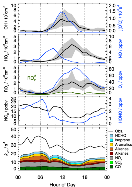
Figure 1 Median diurnal profiles of measured OH, HO 2 , RO 2 , RO 2 # , k_{\text{OH}} , j(\text{O}^1\text{D}) , NO, NO 2 , O 3 , and HONO. For OH, HO 2 and RO 2 , the grey band around the median (black lines) denotes the 25 % and 75 % percentiles of the distributions. In the lowest panel, coloured areas show the speciated reactivity contributions from measured OH reactants.
