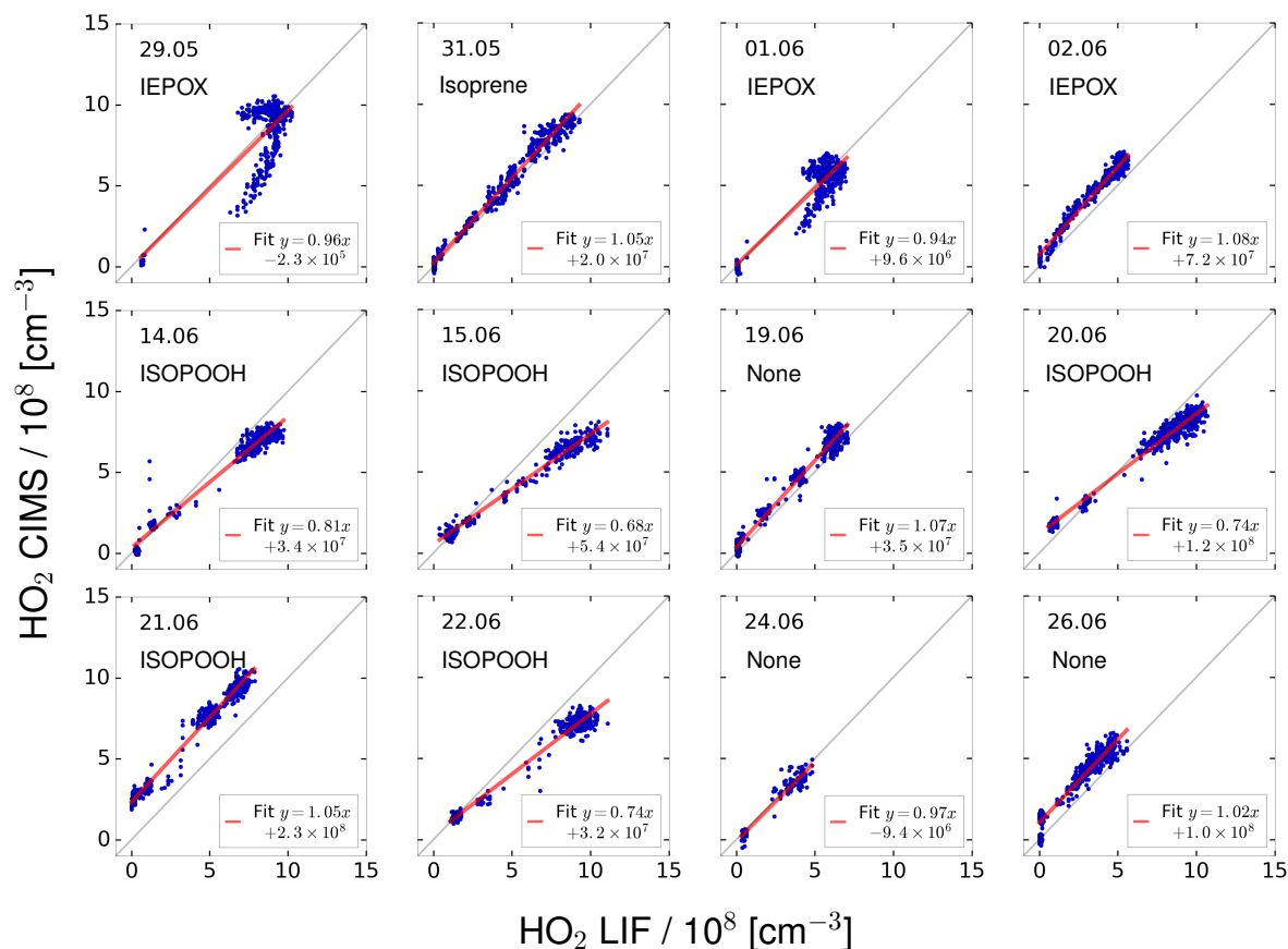
Figure 7. Correlation between HO 2 measurements by the CIMS and LIF instruments for individual chamber experiments. Labels in the plots indicate the specific VOC injected into the chamber.
