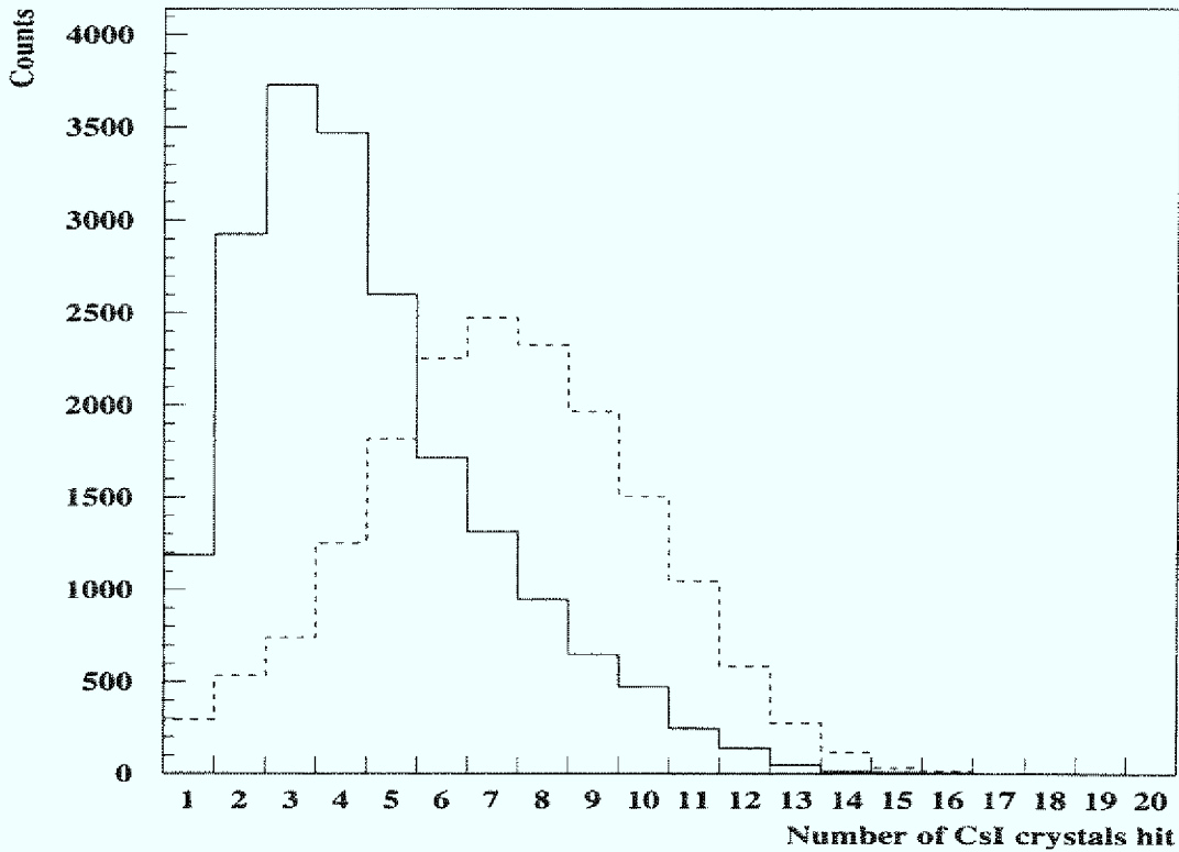
Figure 3.5: Number of CsI crystals hit in one central calorimeter box by absorption of one \eta decay photon (dashed line), respectively \pi^0 decay photon (solid line).
