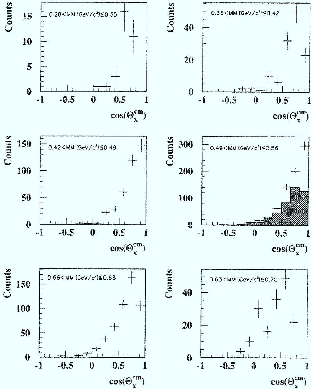
Figure 7.10: Angular distributions (CMS) of the unmeasured rest system in the reaction pd \rightarrow {}^3\text{He}X for six missing mass ranges ( T_p = 1250 MeV).
