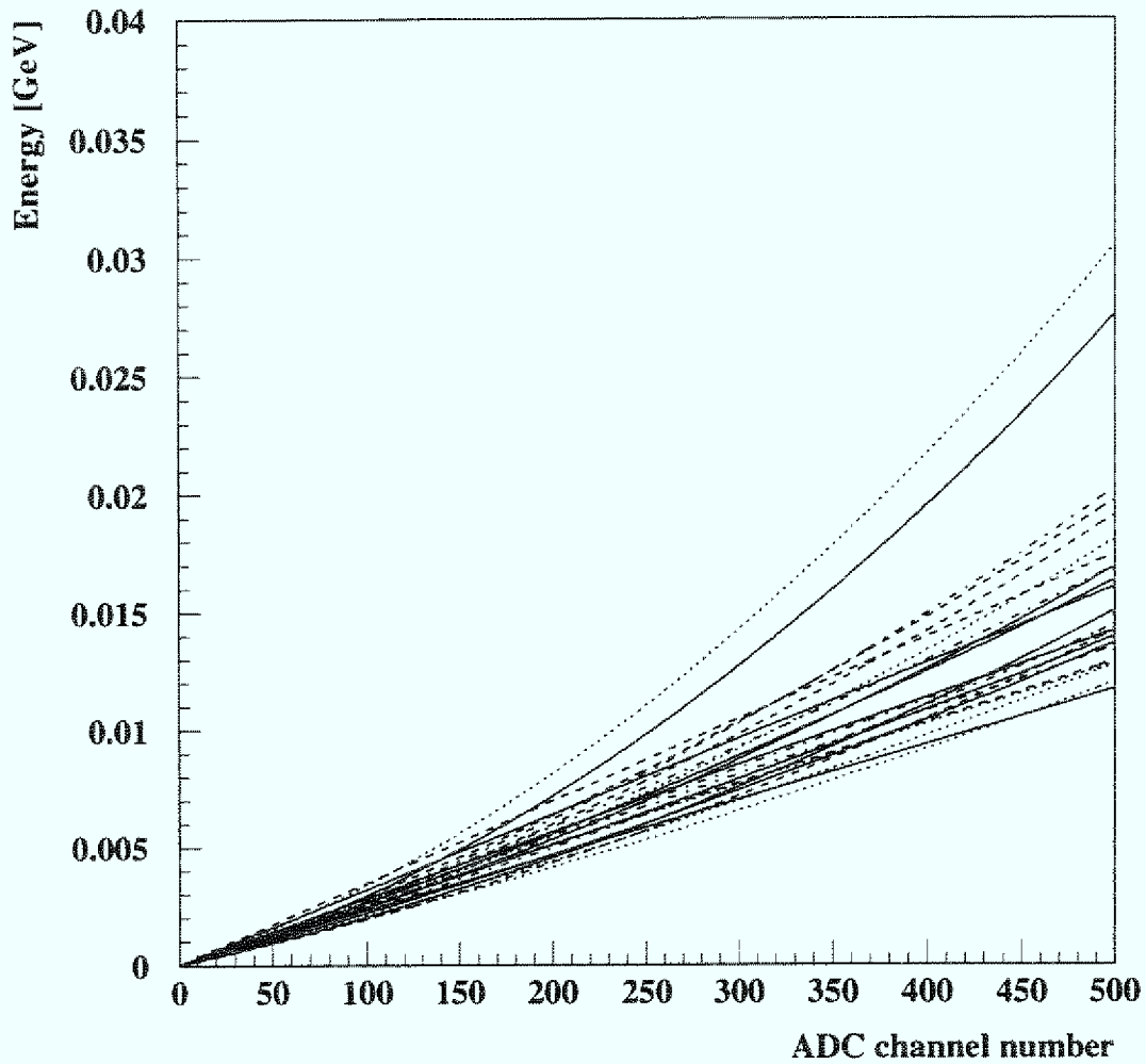
Figure 4.2: ADC to energy calibration curves for all 24 elements of the second forward hodoscope plane.
