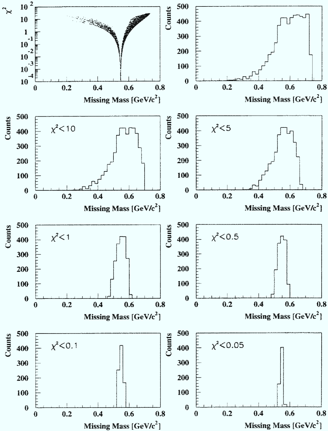
Figure 6.5: \chi^2 versus missing mass for all events (top left), corresponding missing mass spectrum without a cut on \chi^2 (top right), and the same missing mass distribution with stepwise decreased cut on \chi^2 (below) for all events from the reaction pd \rightarrow {}^3\text{He}X at T_p = 1250 MeV.
