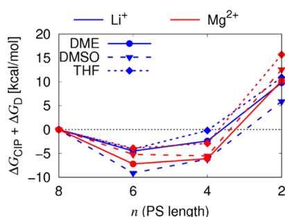
Figure 11. Sum of the change in the contact ion pair formation free energy \Delta G_{CIP} (Figure 9) and the disproportionation free energies \Delta G_D (Figure 10) for Li and Mg polysulfides in larger cation/polysulfide/solvent clusters as a function of the polysulfide chain length n (in terms of monomers). DMSO, THF, and DME have been used as solvents. The reaction free energies of the bare polysulfides were calculated at the G4MP2 level of theory, the contact ion pair formation free energies were calculated at the PBE/6-31+G(d,p) level of theory including a G4MP2 correction (see text for further details).
