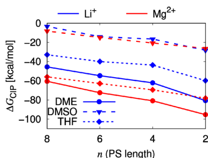
Figure 9. Contact ion pair formation free energies upon bringing a fully solvated \text{Li}^+/\text{Mg}^{2+} ion and a solvated polysulfide anion into contact as a function of the polysulfide chain length n (i.e., in terms of monomers) in different solvents. Blue curves show the free energies for \text{Li}^+ , the red curves show the respective values for \text{Mg}^{2+} . The calculations were performed at the PBE/6-31+G(d,p) level of theory using the implicit SMD solvation model.
