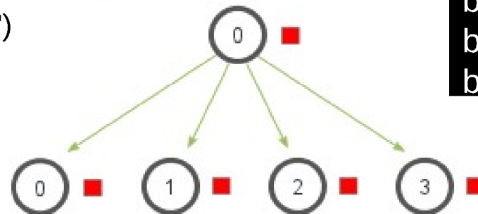
MPI_Bcast
