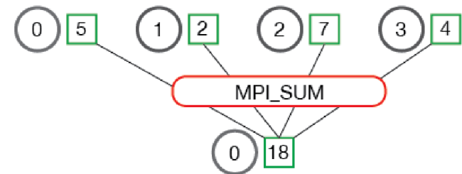
MPI_Reduce
