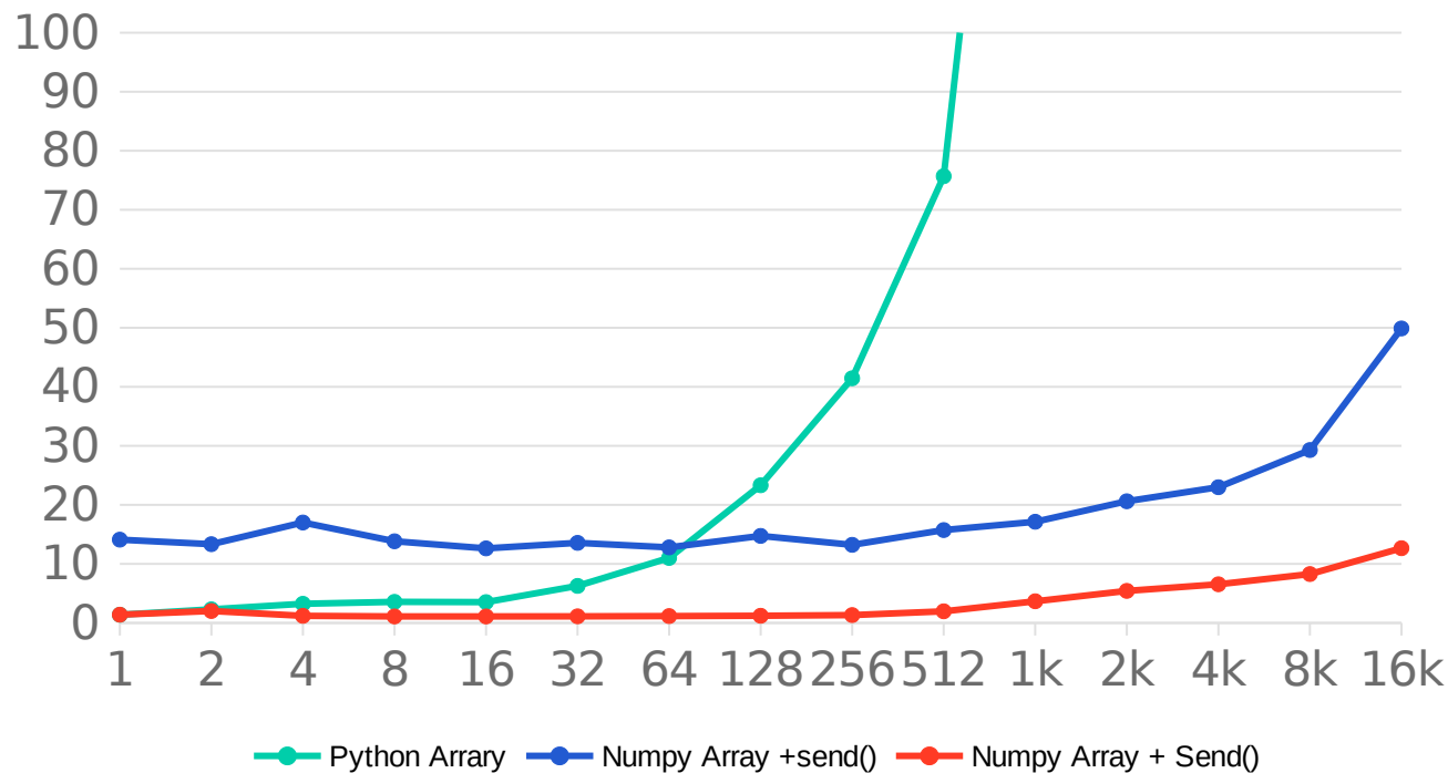
MPI4Py Latency
