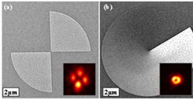
Figure 6. On-axis holograms: (a) Binary phase mask for a Hermite–Gauss mode of 1, 1-like order. (b) Vortex continuous phase mask. Insets: measured beams in the diffraction plane. Reprinted from Shiloh et al (2014) Ultramicroscopy 144 26–31, Copyright (2014), with permission from Elsevier.
