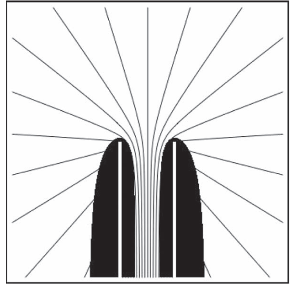
Figure 12. Equiphase lines (black lines) of spacing \pi/4 radians and overlaid amplitude image (black shadows) corresponding to a pair of line charges (white bars) of length 100\ \mu\text{m} and separation 200\ \text{nm} with constant charge densities for C_V = 1 and oppositely charged potentials \pm 2\ \text{V} . Only the tip regions of the line charges are shown in a 1\ \mu\text{m} \times 1\ \mu\text{m} field of view. Reprinted from Pozzi et al (2017) Ultramicroscopy 181 191–196, Copyright (2017), with permission from Elsevier.
