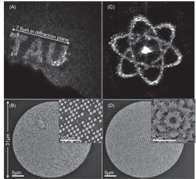
Figure 7. On-axis holograms: (a) ‘TAU’ hologram produced by the mask in (b); Inset: magnification showing \sim 60 nm holes comprising the pixels. (c) Hologram of electrons orbiting a nucleus produced by the mask in (d); Inset: magnification showing the center of the mask. The contrast and brightness levels in (c) were altered for visibility. Reprinted from Shiloh et al (2014) Ultramicroscopy 144 26–31, Copyright (2014), with permission from Elsevier.
