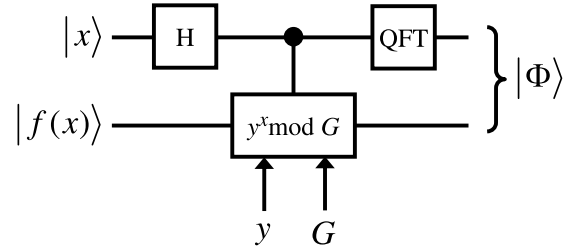
Fig. 5. Schematic diagram of Shor's algorithm.
