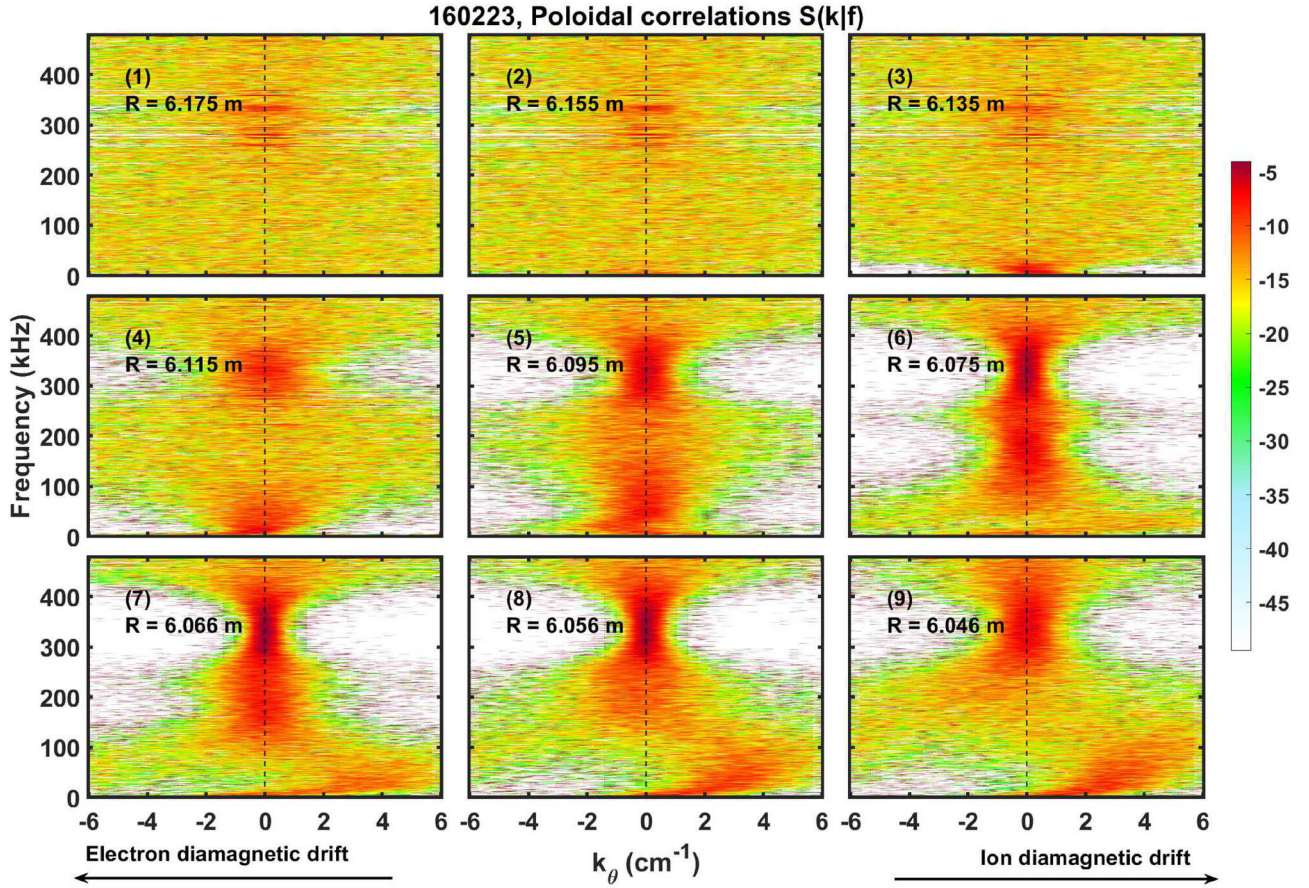
FIG. 8. The poloidal conditional spectral density S(k_\theta|f) of the nine discharges in the experimental day 20160223.
