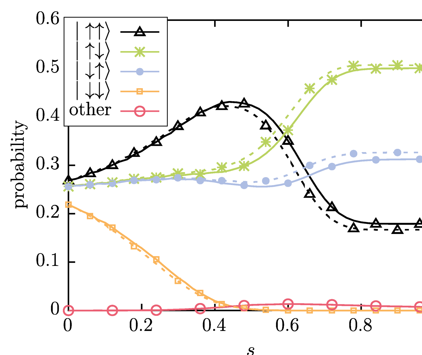
Fig. 2: Probabilities of the basis states during the annealing process for the flux qubits (solid), the ideal 2-level system (dashed) with T_{\text{max}} = 5 ns. Parameters: h_1 = 0.96 , h_2 = 0.94 , J = -1
