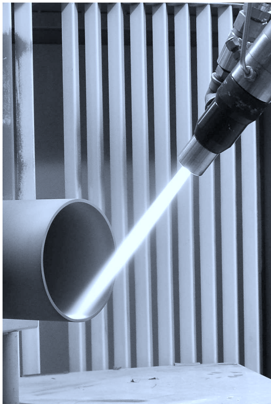
Fig. 1 Off-angle spraying of a tube (internal diameter 160 mm)
