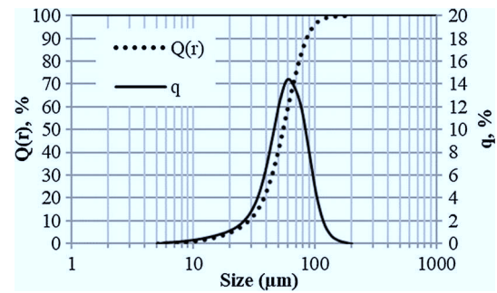
Fig. 4 Particle size distribution of the 7YSZ spray powder
