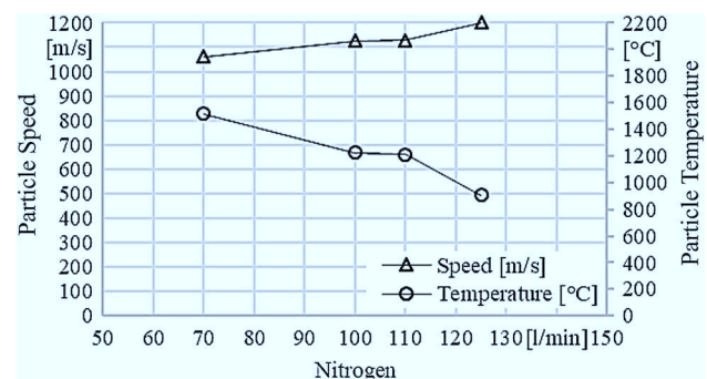
Fig. 6 Particle temperature and particle velocity, measured for parameter SET I with different N_2 volume flow rates
