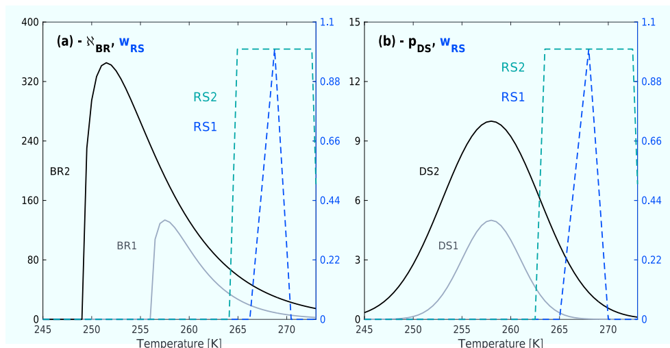
Figure 2. Fragment numbers, weightings, and probabilities from the secondary ice production parameterizations. In panel (a), we show N_{BR} from both ice–ice collisional breakup simulations (BR1 and BR2) as well as the triangular and uniform w_{RS}(T) . In panel (b), we show p_{DS} from both droplet shattering simulations (DS1 and DS2) and w_{RS} once again. The overlapping temperature regions of these are particularly important to understand any feedback between the processes.
