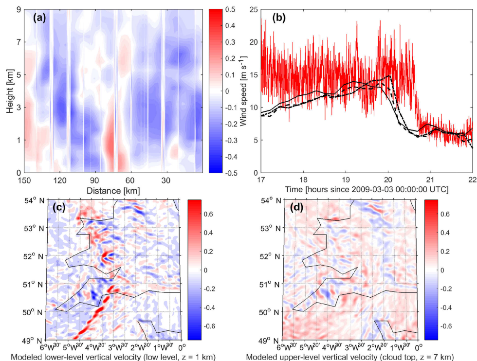
Figure 3. Different model dynamical fields. In panel (a), we show the updraft velocity 150 km along the 255° radial from CFARR at 51.1° N, 1.4° W with values from the CTRL simulation at 19:00 UTC. Discontinuities are due to the minimization of Euclidean distance or interpolation aspects of an algorithm to approximate the radial from the model discretization. Surface wind speeds from 17:00 to 22:00 UTC from the CFARR three cup anemometer and our CTRL simulation are shown in panel (b). Panels (c) and (d) show the modeled vertical velocities from the CTRL simulation at 1 and 7 km, respectively, at 18:00 UTC as the rainband began to pass over the UK.
