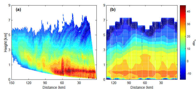
Figure 4. Model-measurement intercomparison of range-height indicator scans of radar reflectivity Z_{DH} along the 255° radial out from CFARR. CAMRa Doppler radar measurements are shown in panel (a) for the scan taken between 19:22:07 and 19:23:07 UTC, and modeled values are shown from the CTRL simulation at 19:00:00 UTC, both in dBZ h .
