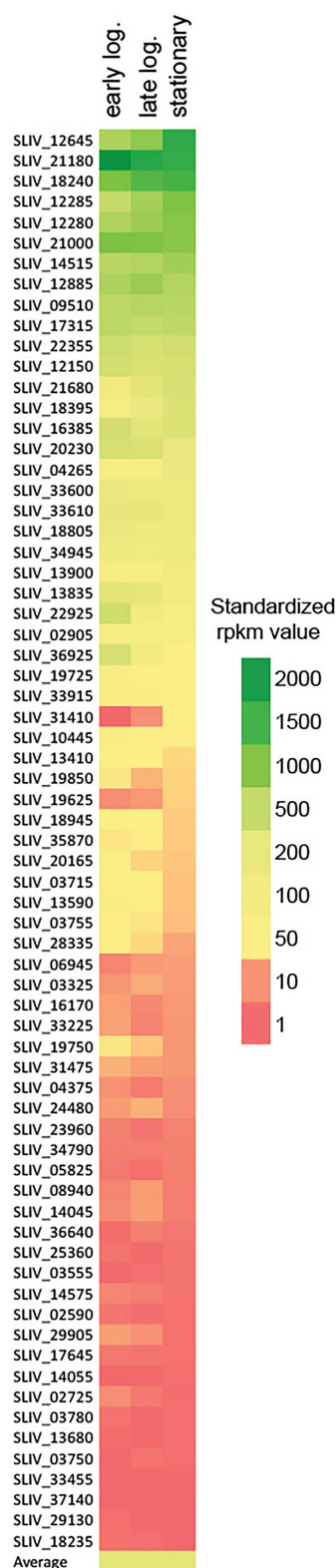
FIGURE 2 | Heat-map of transcription levels of sigma factor coding genes in S. lividans TK24 culture at earlier and late logarithmic and stationary phases of growth. The average rpkm is shown to estimate the overall transcriptional activity of the genome under tested conditions.
