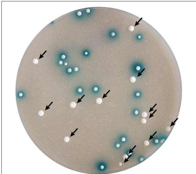
FIGURE 3 | Selection of secondary cross-over mutants of S. lividans with the use of gusA -based BAC clones. Plates after conjugation were overlaid with the X-gluc solution. Blue colonies carry the single cross-over inserted recombinant BAC clone; white colonies originated from secondary cross-over event eliminating the vector backbone and thus resulting in replacement of target gene with the antibiotic resistance cassette.
