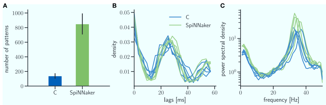
FIGURE 9 | Frequency and structure of spatiotemporal spike patterns. (A) Bar diagram of the number of patterns detected using the SPADE method (Quaglio et al., 2017) in the two simulations. Displayed are the mean and standard deviation of the results for the 5 network states. The spike times of all 800 excitatory neurons are discretized by 3 ms bins and only spike sequences that repeated 3 or more times, are formed by at least 5 spikes, and with a temporal length between first and last spike shorter than 60 ms are considered. (B) Normalized distributions of the temporal lags between any two spikes involved in one of the patterns. The results for each of the 5 network states are displayed as a separate distribution. (C) Power spectra of the population activity in each network state. The spectra are calculated by Welch's method with a 100 Hz sampling frequency and a 1 Hz frequency resolution (window overlap: 50%). In all panels, data from the C and SpiNNaker simulations are indicated in blue and green, respectively.
