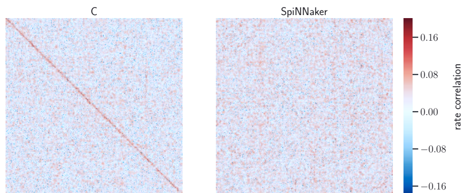
FIGURE 8 | Rate-correlation matrices for the C and SpiNNaker simulations of the network state after 5 h. Matrix elements show the RCs (color bar) of all pairs the 800 excitatory model neurons in the simulation computed from 60 s of data. The order of the neuron ids in both symmetric matrices is determined by hierarchical clustering (Ward's variance minimization algorithm, details see Section 3.1.3) of the C matrix. Auto-correlations are set to 0 to not stretch the color scale.
