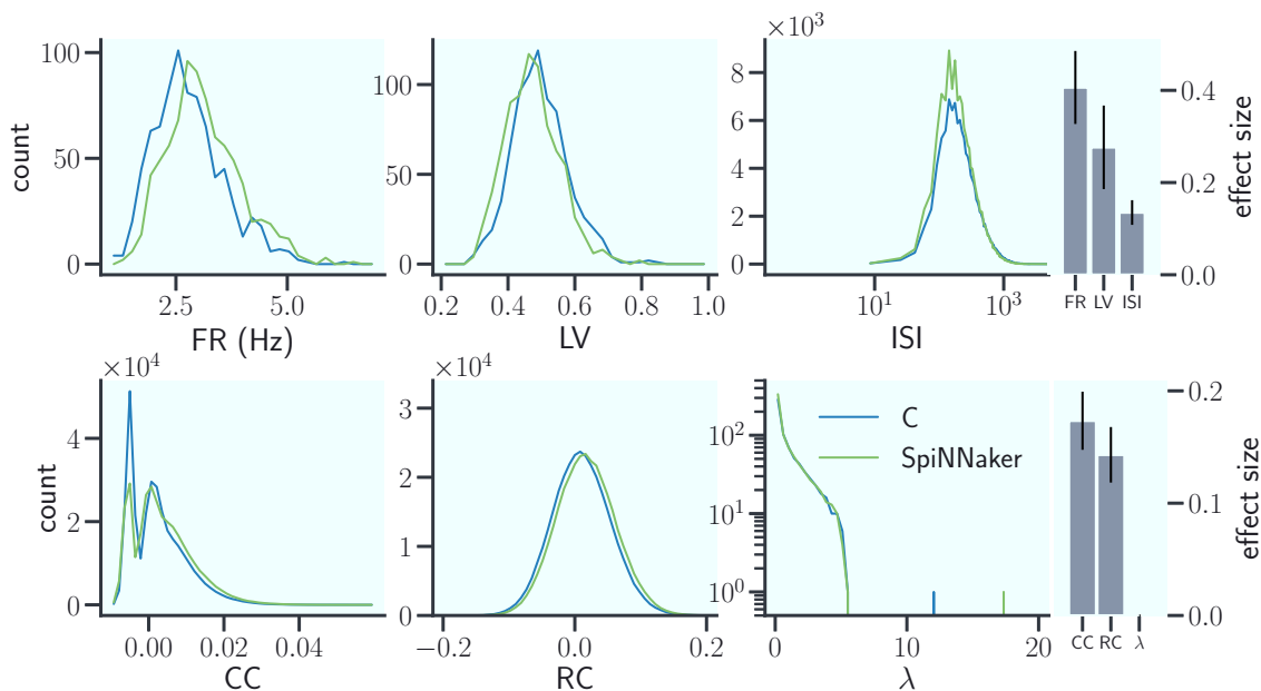
FIGURE 7 | Distributions of characteristic measures of network activity simulated with C and SpiNNaker after the final step of refinement. The top row shows single neuron statistics FR, LV, and the ISIs (same display and data specification as in Figure 5B ). The histograms of ISIs are displayed using semi-logarithmic scaling. The bottom row shows pairwise statistics and network properties, namely the CC using 2 ms bins, the rate correlation (RC) using 100 ms bins, and the eigenvalues ( \lambda ) of the RC matrices displayed on the vertical axis using a logarithmic scaling. Right: effect size using the same display as in Figure 6 . The effect sizes for the tested measures are FR: 0.41 \pm 0.08 , LV: 0.28 \pm 0.09 , ISI: 0.14 \pm 0.03 , CC: 0.17 \pm 0.03 , RC: 0.14 \pm 0.02 , and \lambda : < 8 \times 10^{-17} , respectively.
