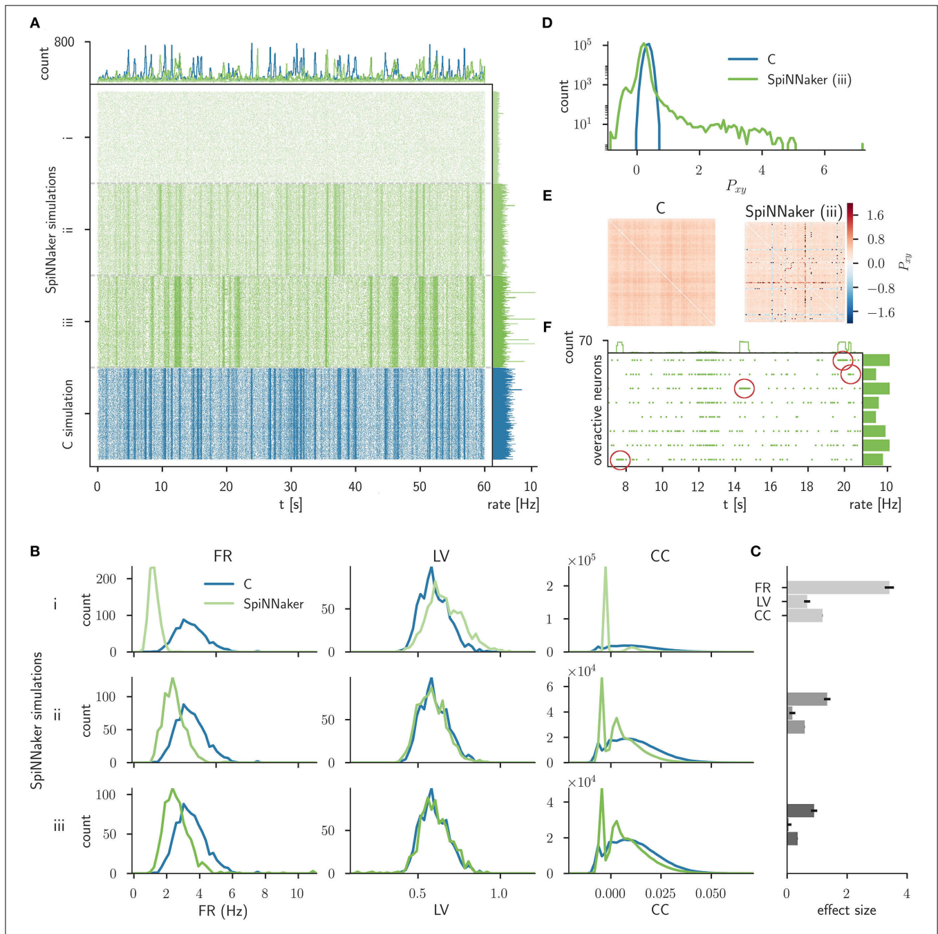
FIGURE 5 | Comparison of the C simulation with simulations of three consecutive stages of the SpiNNaker implementation. (A) Raster plot of the spiking network activity (800 excitatory neurons) of the C simulation (bottom, blue) and three stages of the SpiNNaker implementation; i, ii, and iii (top, shades of green). The top and right histograms show the population spike counts in 60 ms bins and the mean firing rates, respectively. (B) Distributions of firing rates (FR, left), local coefficients of variation (LV, middle), and correlation coefficients (CC, right) for the C and SpiNNaker simulations. Each row (subsequent implementation steps: i, ii, iii) represents a specific SpiNNaker simulation (green) that differs in the underlying neuron model implementation. Data shown for the C simulation (blue) are identical in the three rows. (C) The difference between the distributions is quantified by the effect size with error bars indicating the 95% confidence interval. In step iii the effect sizes for the FR, LV, and CC measure are 0.90, 0.05, and 0.36, respectively. (D) Distributions of the sum of the cross-correlation coefficient ( P_{xy} , Equation 7) in logarithmic representation for C and SpiNNaker (implementation step iii). (E) Color coded correlation matrices for the sum of the cross-correlation coefficient in implementation step iii. The symmetric matrices display results for the subset of 100 excitatory neurons with highest spike rates in the SpiNNaker simulation. (F) Raster plot of 8 overactive neurons in the SpiNNaker simulation (implementation step iii) showing episodes of 1 kHz spiking (emphasized by red markers). The top and right histograms show the population spike counts in 60 ms bins and the mean firing rates for the entire recording, respectively.
