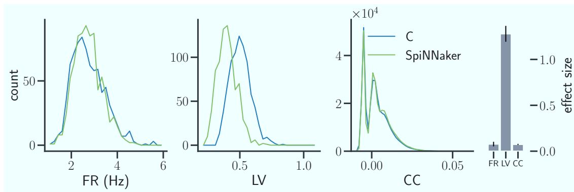
FIGURE 6 | Comparison of statistical measures after model refinement. The panels show from left to right the distributions of FR, LV, and CC of the C and SpiNNaker simulation after the first refinement of the implementations by Trensch et al. (2018) for the network state after t_5 = 5 h (same display as in Figure 5B ). The histogram on the right visualizes the effect size in the three statistical measures (mean and standard deviation across all five network states t_1, t_2, \dots, t_5 ). The numerical values are FR: 0.077 \pm 0.025 , LV: 1.28 \pm 0.086 , and CC: 0.074 \pm 0.006 respectively.
