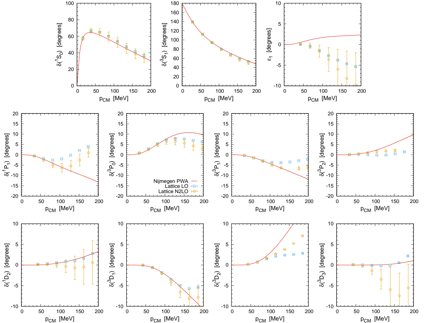
FIG. 2: LO (squares) and NNLO (circles) neutron-proton phase shifts and mixing angles for a = 1.64 fm. The NPWA is given by the solid line.
