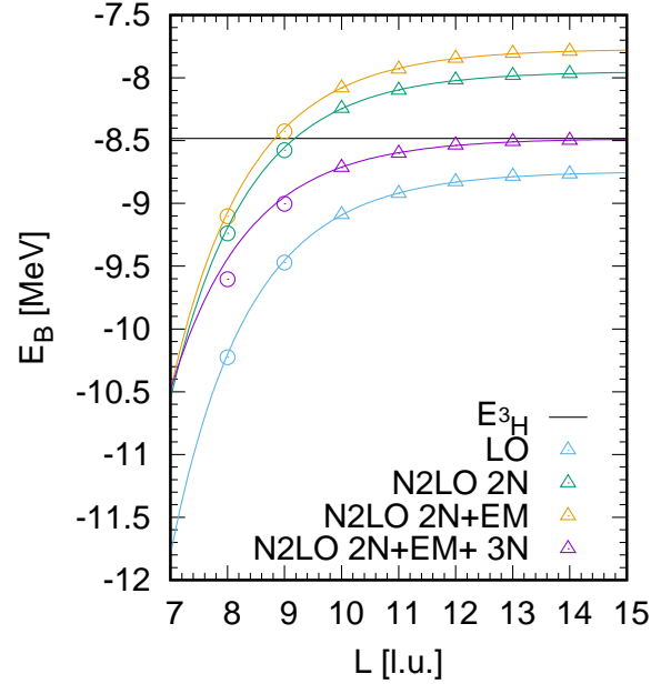
FIG. 5: Finite volume extrapolation for the triton and a lattice spacing of a = 1.32 fm. The triangles are included in the fit while the circles are not due to higher order finite volume effects.
