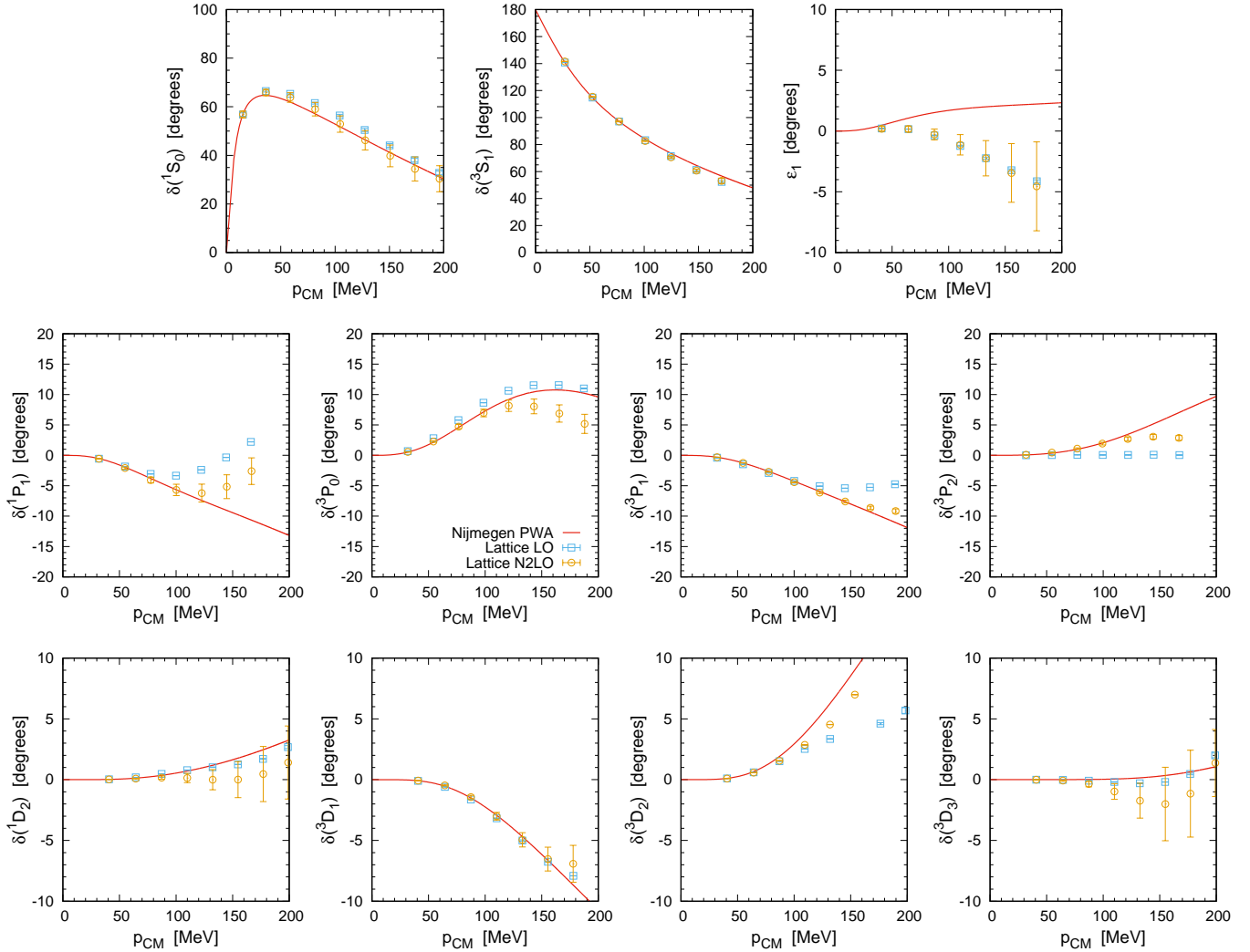
FIG. 3: LO (squares) and NNLO (circles) neutron-proton phase shifts and mixing angles for a = 1.32 fm. The NPWA is given by the solid line.
