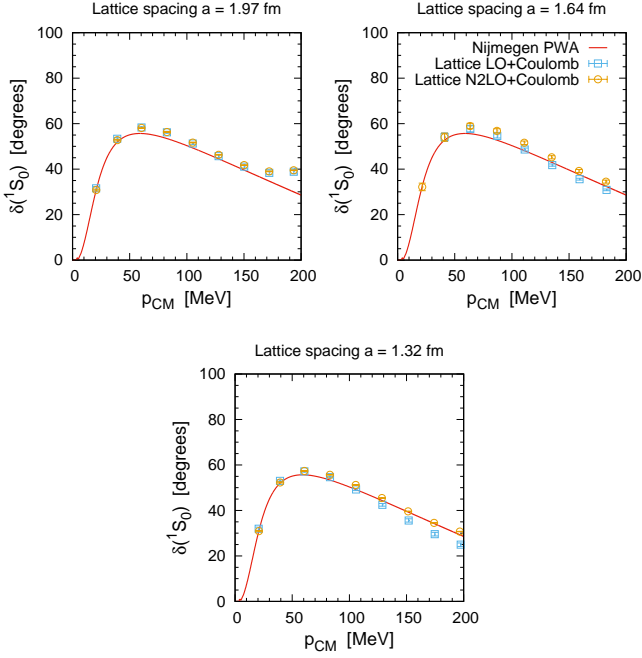
FIG. 4: LO (squares) and NNLO (circles) (both including Coulomb) proton-proton ^1S_0 phase shift for a = 1.97 fm, a = 1.64 fm and a = 1.32 fm. The NPWA is given by the solid line.
